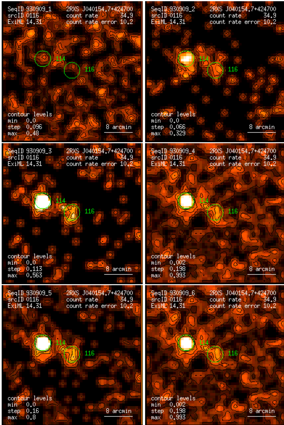
Figure 116: RASS 930909: detection 0116: band rate images, Gaussian filter: (1) PSPC channels 11 – 41, (2) 52 – 90, (3) 91 – 201, (4) 11 – 235, (5) 52 – 201, (6) 11 – 201. Broad band rates in counts/ks. Band rate contour levels in counts/ks/arcmin 2 .
