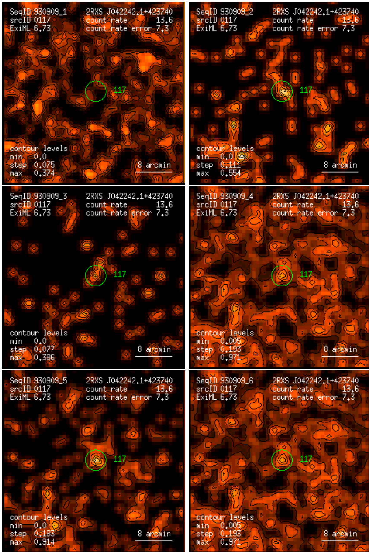
Figure 117: RASS 930909: detection 0117: band rate images, Gaussian filter: (1) PSPC channels 11 – 41, (2) 52 – 90, (3) 91 – 201, (4) 11 – 235, (5) 52 – 201, (6) 11 – 201. Broad band rates in counts/ks. Band rate contour levels in counts/ks/arcmin 2 .
