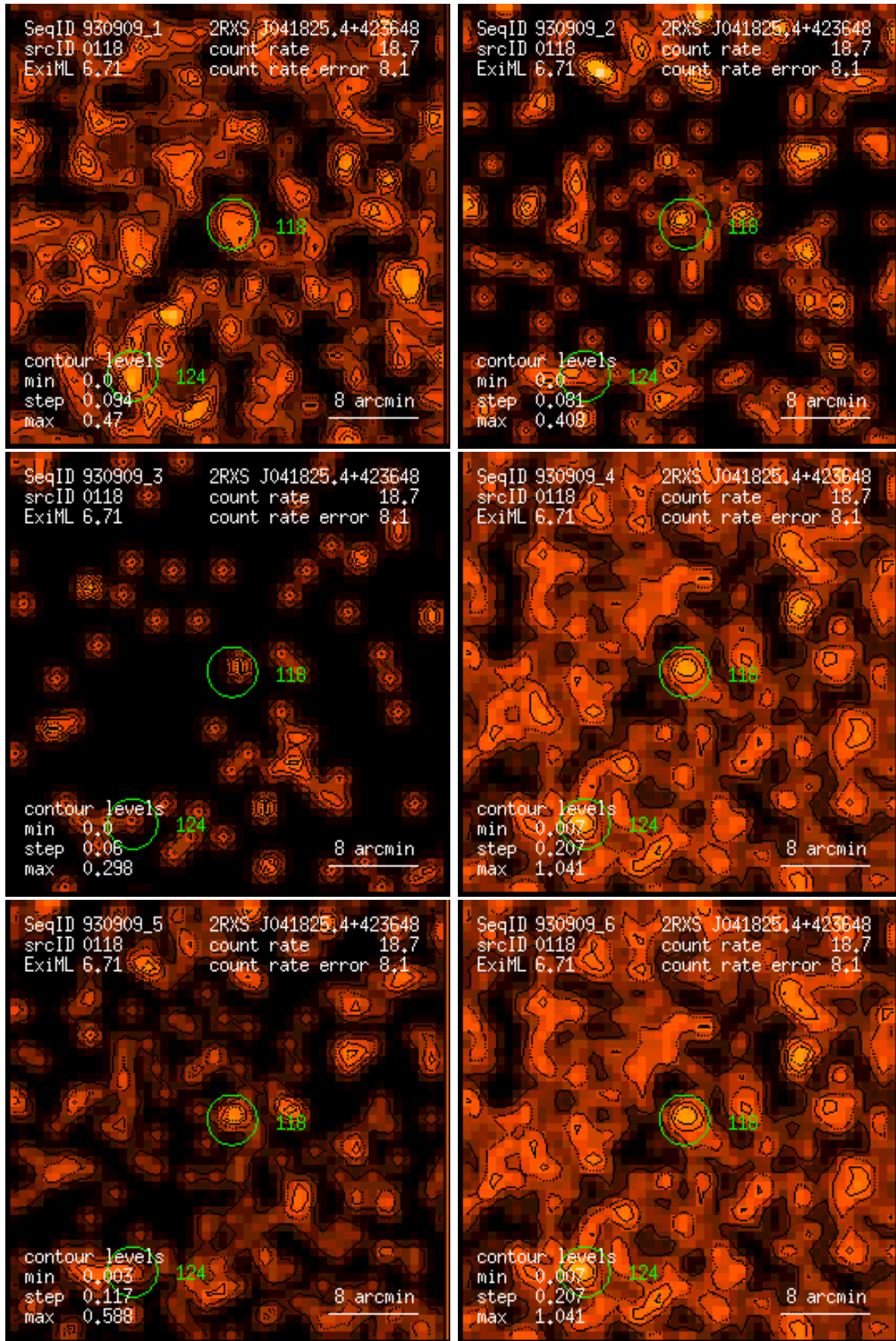
Figure 118: RASS 930909: detection 0118: band rate images, Gaussian filter: (1) PSPC channels 11 – 41, (2) 52 – 90, (3) 91 – 201, (4) 11 – 235, (5) 52 – 201, (6) 11 – 201. Broad band rates in counts/ks. Band rate contour levels in counts/ks/arcmin 2 .
