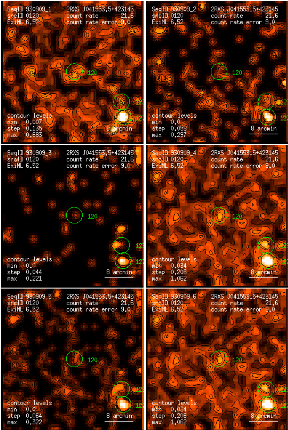
Figure 120: RASS 930909: detection 0120: band rate images, Gaussian filter: (1) PSPC channels 11 – 41, (2) 52 – 90, (3) 91 – 201, (4) 11 – 235, (5) 52 – 201, (6) 11 – 201. Broad band rates in counts/ks. Band rate contour levels in counts/ks/arcmin 2 .
