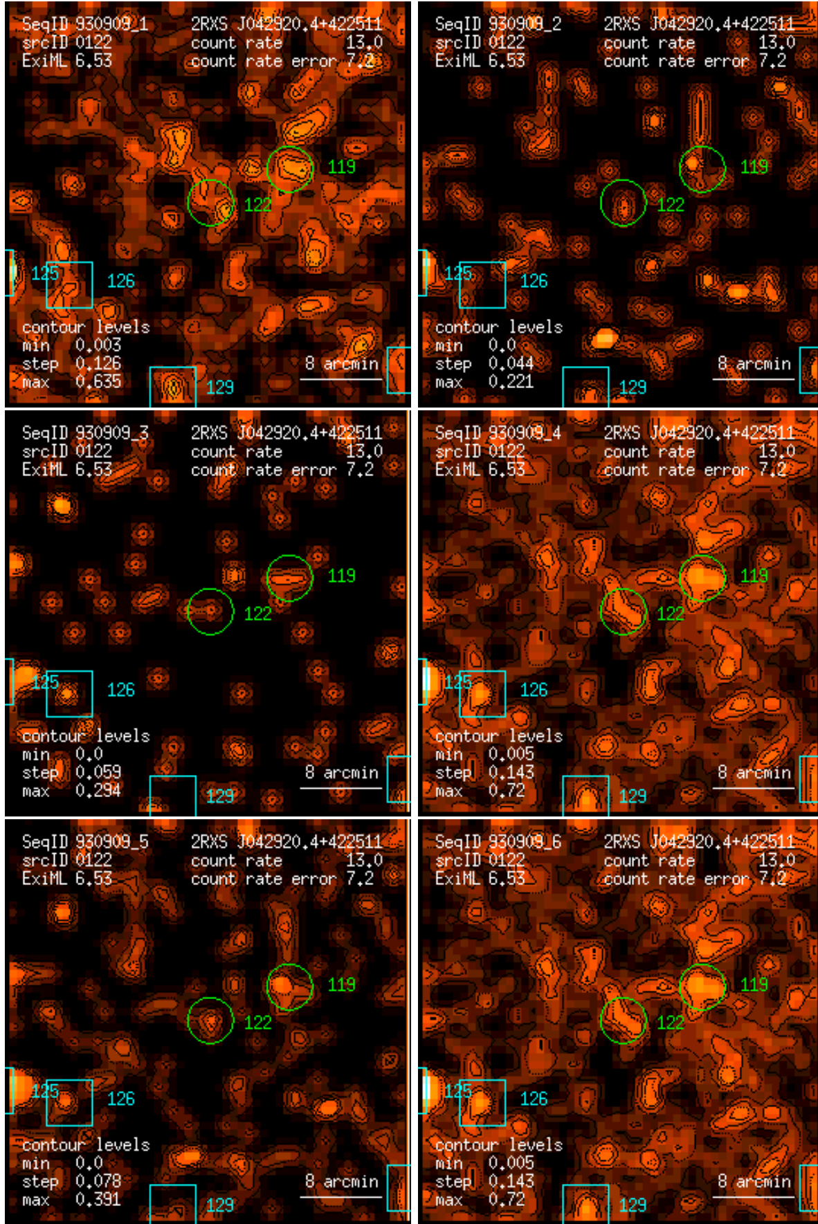
Figure 122: RASS 930909: detection 0122: band rate images, Gaussian filter: (1) PSPC channels 11 – 41, (2) 52 – 90, (3) 91 – 201, (4) 11 – 235, (5) 52 – 201, (6) 11 – 201. Broad band rates in counts/ks. Band rate contour levels in counts/ks/arcmin 2 .
