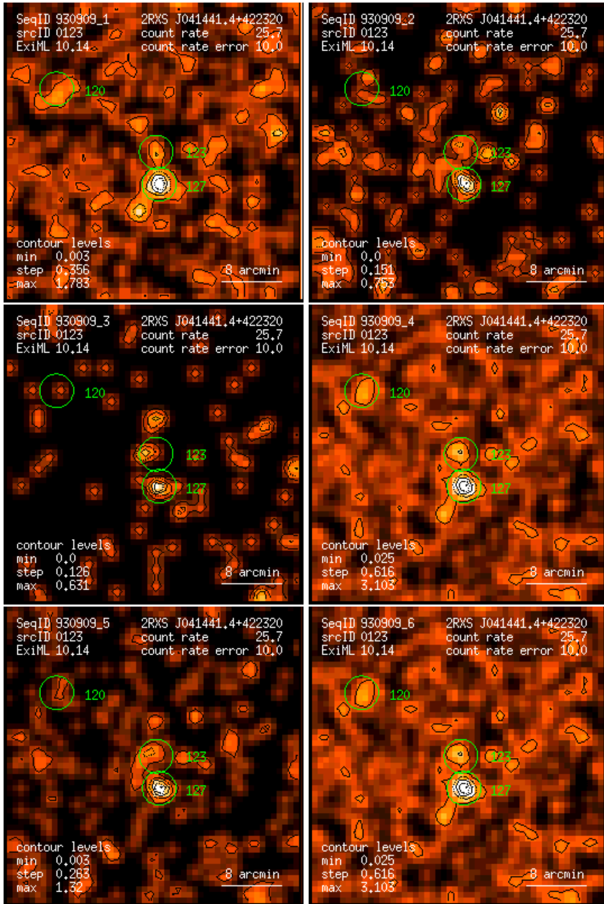
Figure 123: RASS 930909: detection 0123: band rate images, Gaussian filter: (1) PSPC channels 11 – 41, (2) 52 – 90, (3) 91 – 201, (4) 11 – 235, (5) 52 – 201, (6) 11 – 201. Broad band rates in counts/ks. Band rate contour levels in counts/ks/arcmin 2 .
