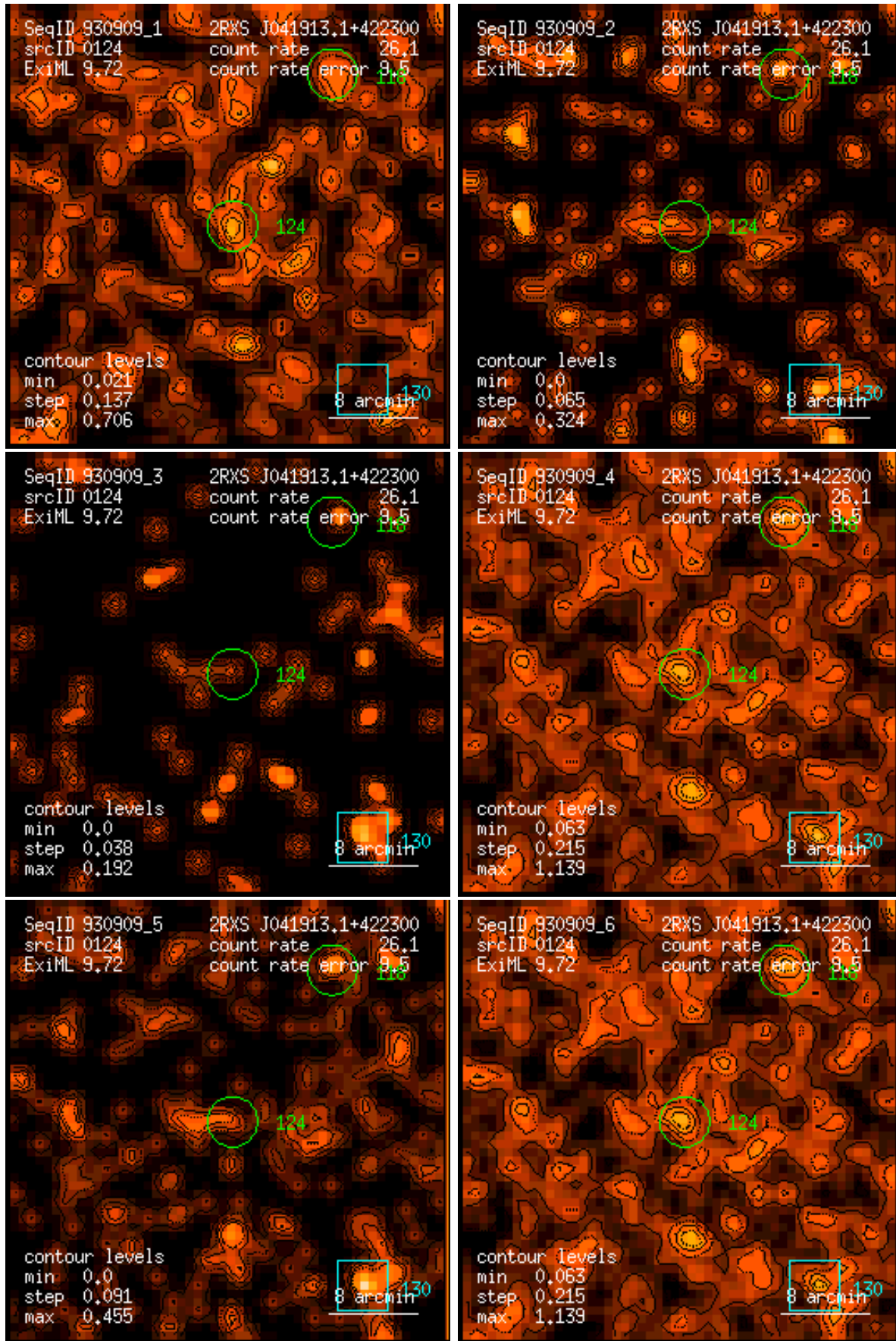
Figure 124: RASS 930909: detection 0124: band rate images, Gaussian filter: (1) PSPC channels 11 – 41, (2) 52 – 90, (3) 91 – 201, (4) 11 – 235, (5) 52 – 201, (6) 11 – 201. Broad band rates in counts/ks. Band rate contour levels in counts/ks/arcmin 2 .
