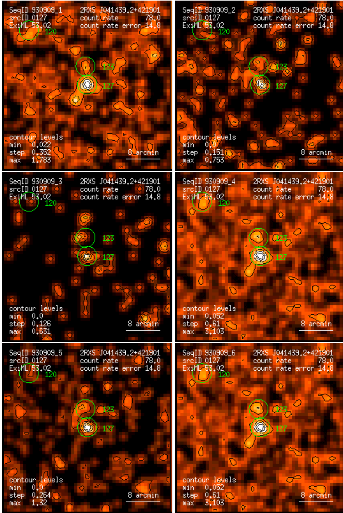
Figure 127: RASS 930909: detection 0127: band rate images, Gaussian filter: (1) PSPC channels 11 – 41, (2) 52 – 90, (3) 91 – 201, (4) 11 – 235, (5) 52 – 201, (6) 11 – 201. Broad band rates in counts/ks. Band rate contour levels in counts/ks/arcmin 2 .
