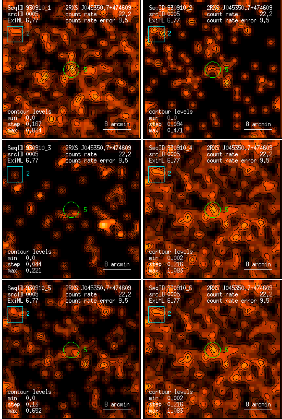
Figure 5: RASS 930910: detection 0005: band rate images, Gaussian filter: (1) PSPC channels 11 – 41, (2) 52 – 90, (3) 91 – 201, (4) 11 – 235, (5) 52 – 201, (6) 11 – 201. Broad band rates in counts/ks. Band rate contour levels in counts/ks/arcmin 2 .
