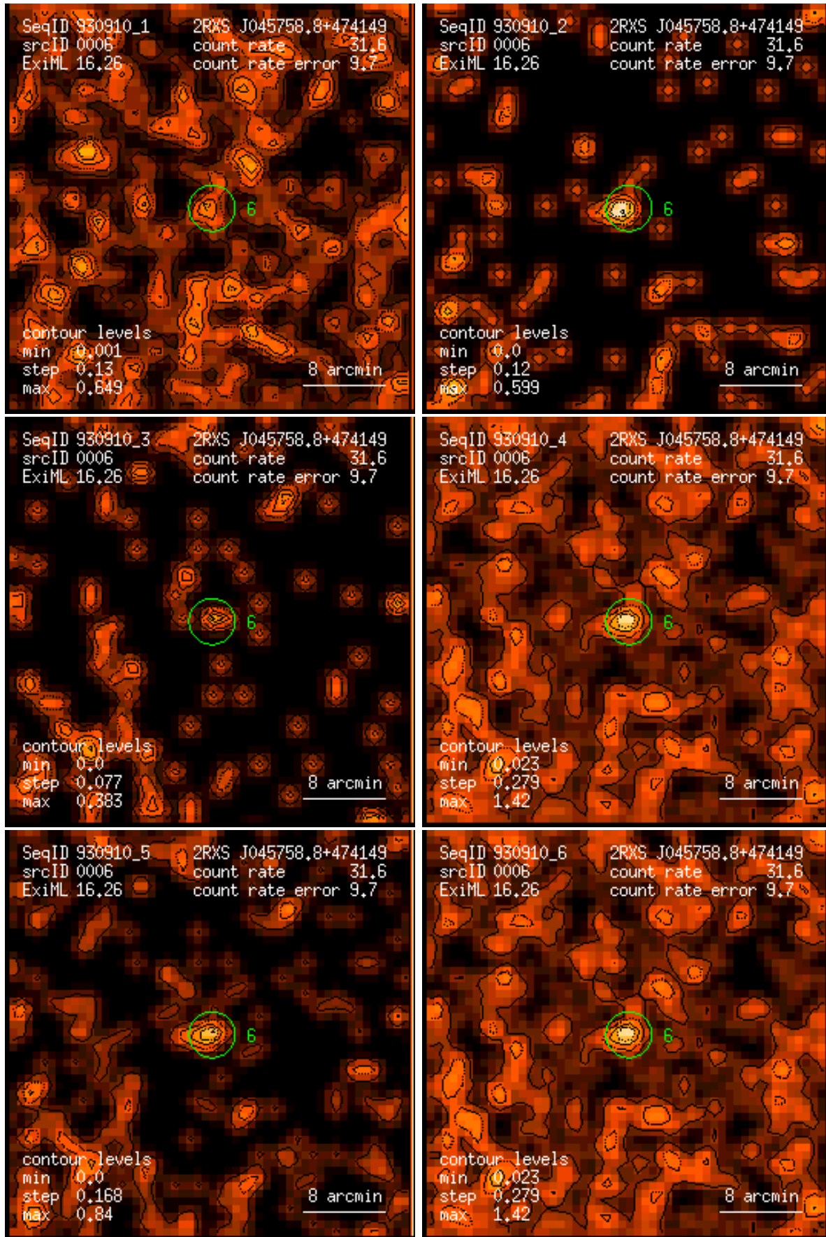
Figure 6: RASS 930910: detection 0006: band rate images, Gaussian filter: (1) PSPC channels 11 – 41, (2) 52 – 90, (3) 91 – 201, (4) 11 – 235, (5) 52 – 201, (6) 11 – 201. Broad band rates in counts/ks. Band rate contour levels in counts/ks/arcmin 2 .
