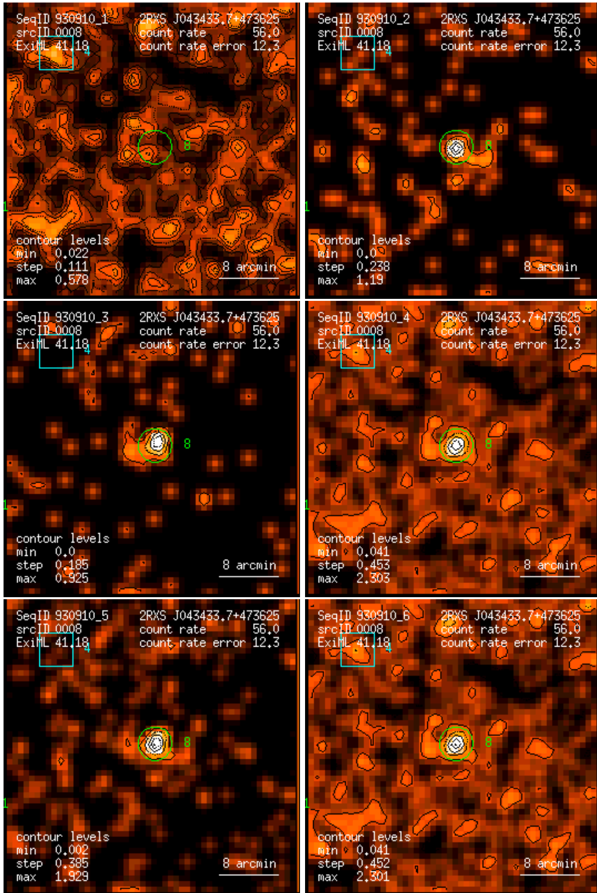
Figure 8: RASS 930910: detection 0008: band rate images, Gaussian filter: (1) PSPC channels 11 – 41, (2) 52 – 90, (3) 91 – 201, (4) 11 – 235, (5) 52 – 201, (6) 11 – 201. Broad band rates in counts/ks. Band rate contour levels in counts/ks/arcmin 2 .
