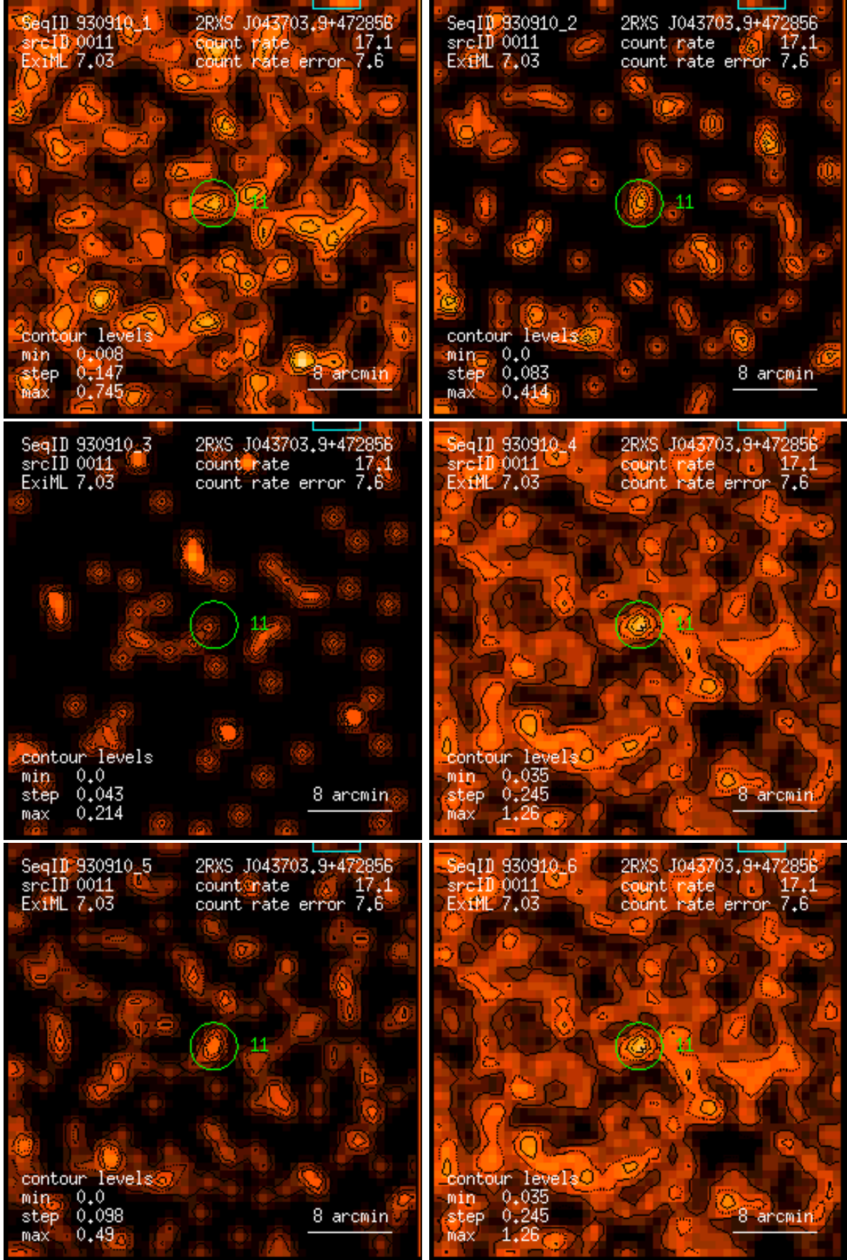
Figure 11: RASS 930910: detection 0011: band rate images, Gaussian filter: (1) PSPC channels 11 – 41, (2) 52 – 90, (3) 91 – 201, (4) 11 – 235, (5) 52 – 201, (6) 11 – 201. Broad band rates in counts/ks. Band rate contour levels in counts/ks/arcmin 2 .
