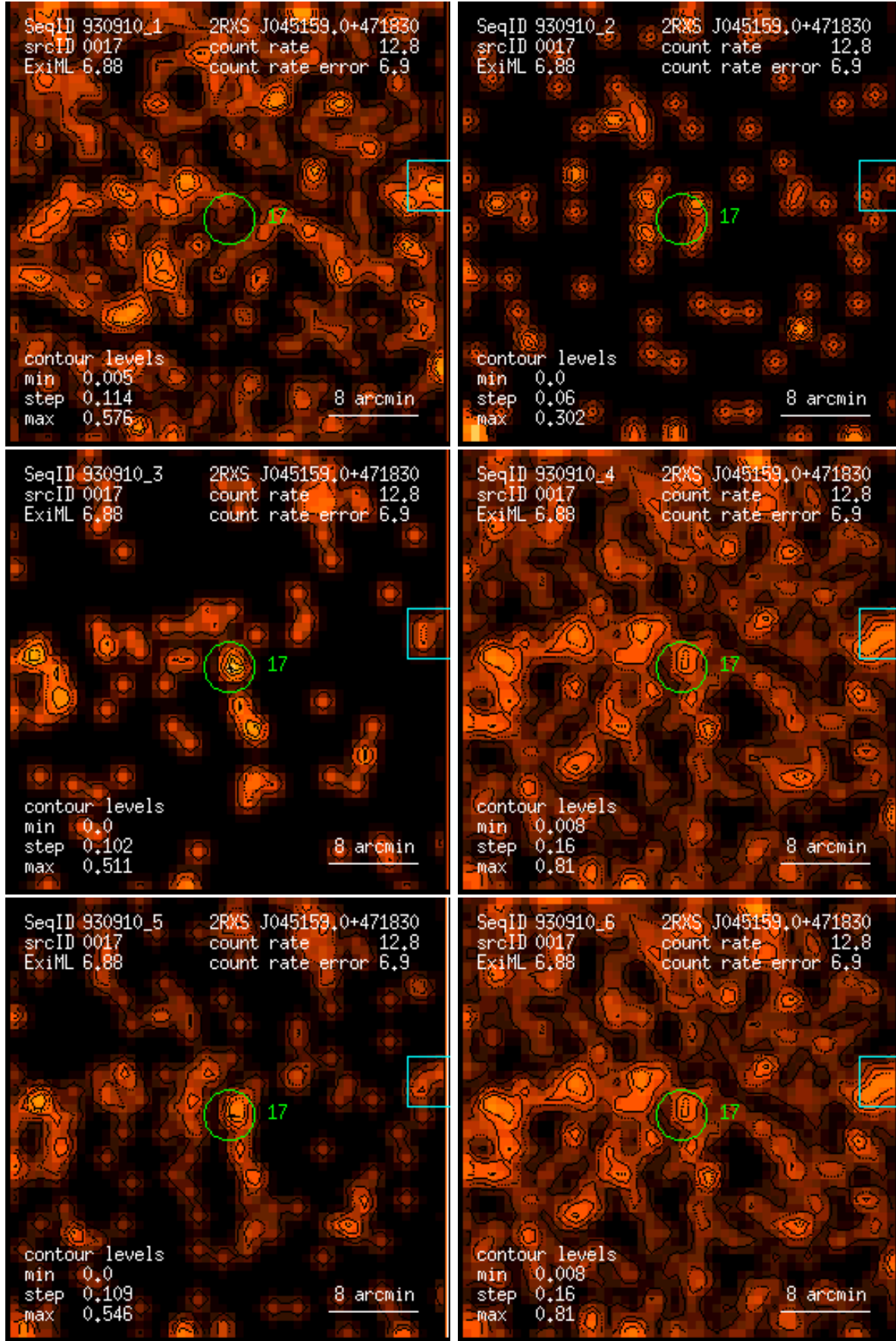
Figure 17: RASS 930910: detection 0017: band rate images, Gaussian filter: (1) PSPC channels 11 – 41, (2) 52 – 90, (3) 91 – 201, (4) 11 – 235, (5) 52 – 201, (6) 11 – 201. Broad band rates in counts/ks. Band rate contour levels in counts/ks/arcmin 2 .
