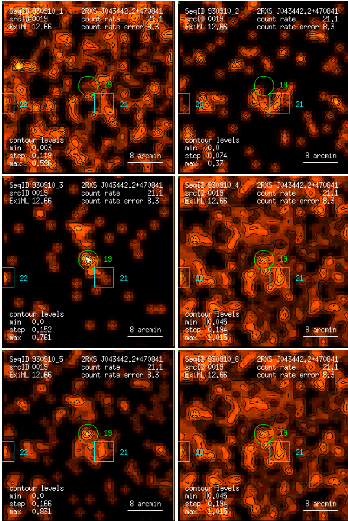
Figure 19: RASS 930910: detection 0019: band rate images, Gaussian filter: (1) PSPC channels 11 – 41, (2) 52 – 90, (3) 91 – 201, (4) 11 – 235, (5) 52 – 201, (6) 11 – 201. Broad band rates in counts/ks. Band rate contour levels in counts/ks/arcmin 2 .
