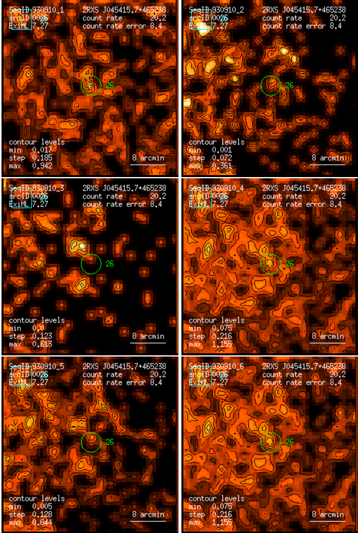
Figure 26: RASS 930910: detection 0026: band rate images, Gaussian filter: (1) PSPC channels 11 – 41, (2) 52 – 90, (3) 91 – 201, (4) 11 – 235, (5) 52 – 201, (6) 11 – 201. Broad band rates in counts/ks. Band rate contour levels in counts/ks/arcmin 2 .
