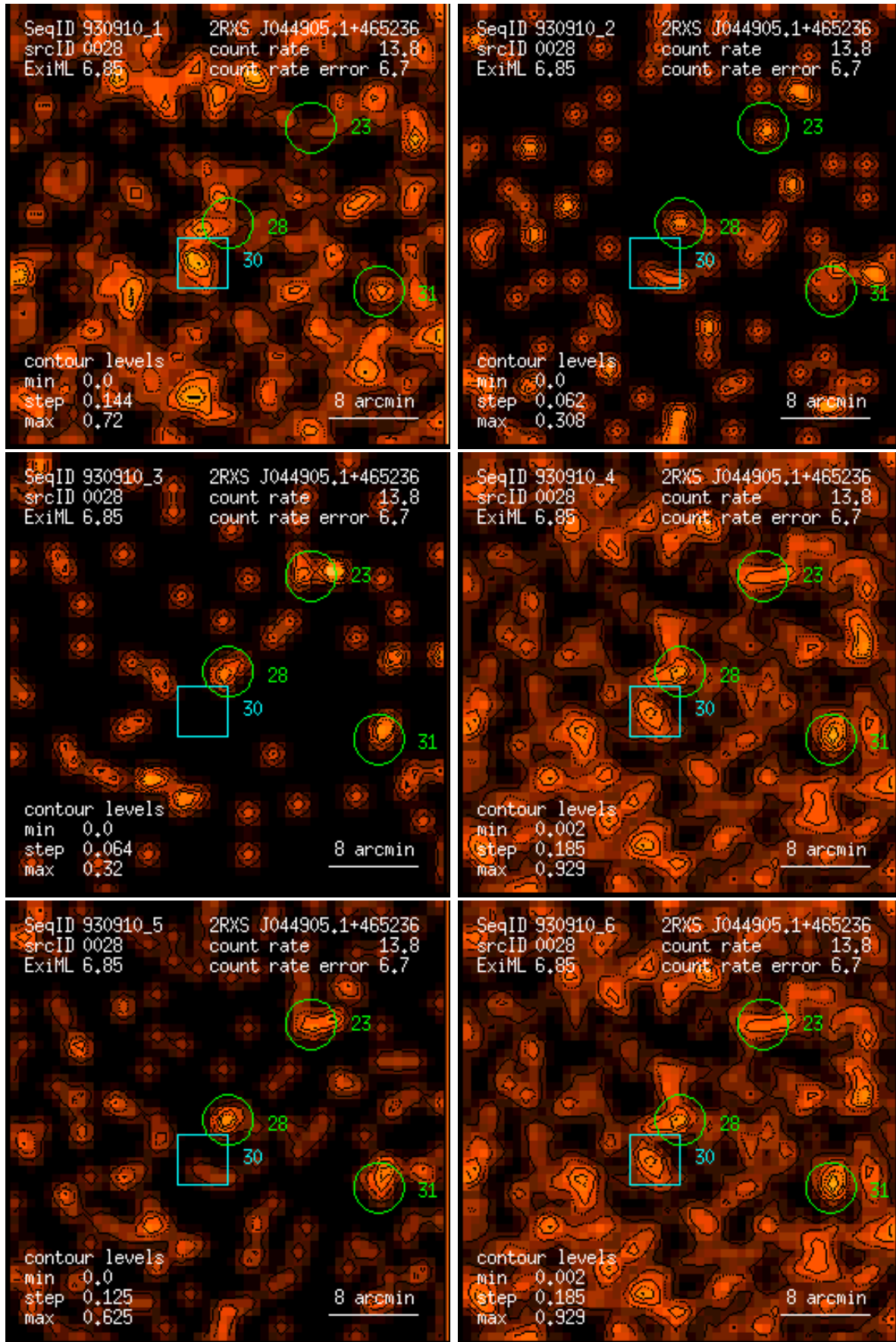
Figure 28: RASS 930910: detection 0028: band rate images, Gaussian filter: (1) PSPC channels 11 – 41, (2) 52 – 90, (3) 91 – 201, (4) 11 – 235, (5) 52 – 201, (6) 11 – 201. Broad band rates in counts/ks. Band rate contour levels in counts/ks/arcmin 2 .
