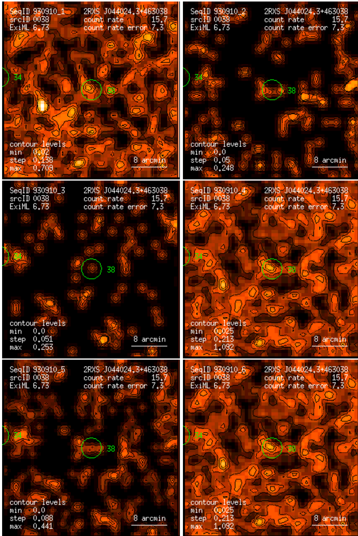
Figure 38: RASS 930910: detection 0038: band rate images, Gaussian filter: (1) PSPC channels 11 – 41, (2) 52 – 90, (3) 91 – 201, (4) 11 – 235, (5) 52 – 201, (6) 11 – 201. Broad band rates in counts/ks. Band rate contour levels in counts/ks/arcmin 2 .
