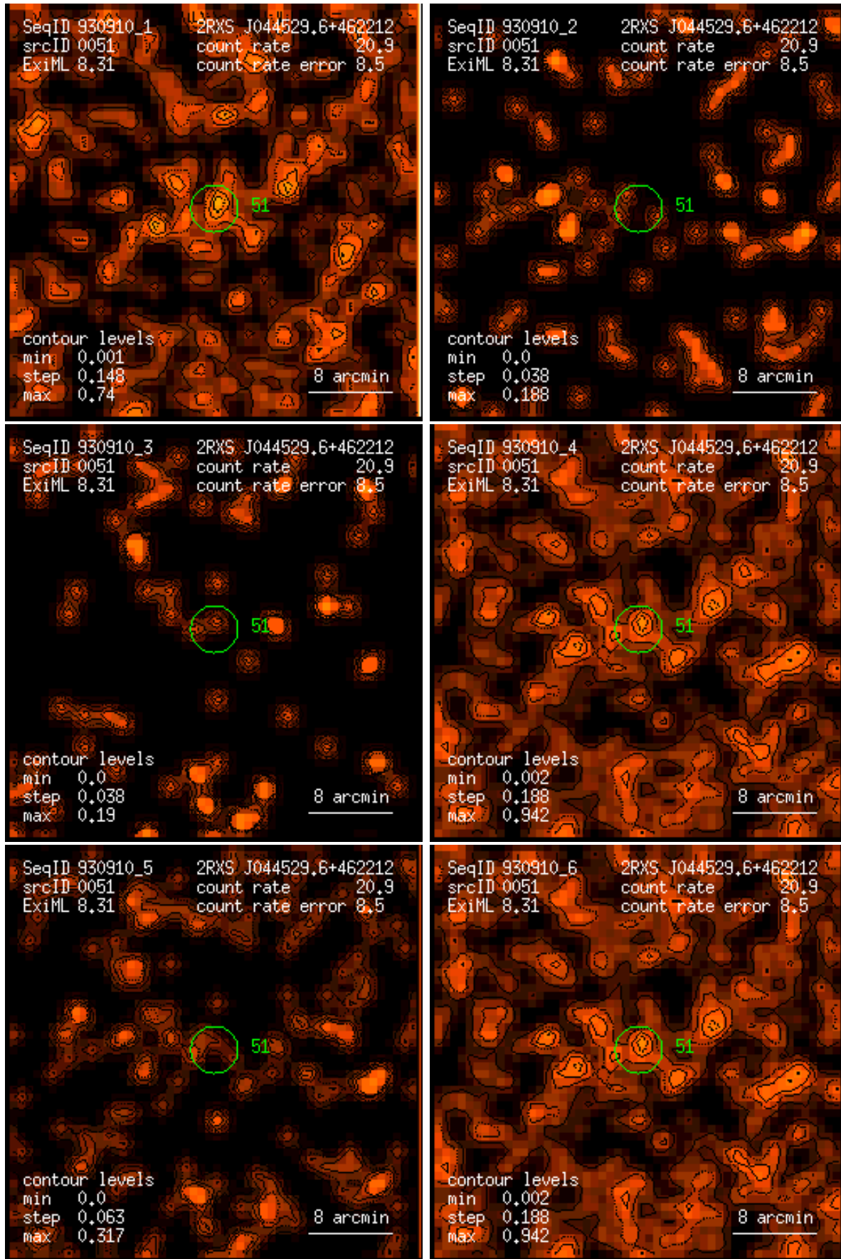
Figure 51: RASS 930910: detection 0051: band rate images, Gaussian filter: (1) PSPC channels 11 – 41, (2) 52 – 90, (3) 91 – 201, (4) 11 – 235, (5) 52 – 201, (6) 11 – 201. Broad band rates in counts/ks. Band rate contour levels in counts/ks/arcmin 2 .
