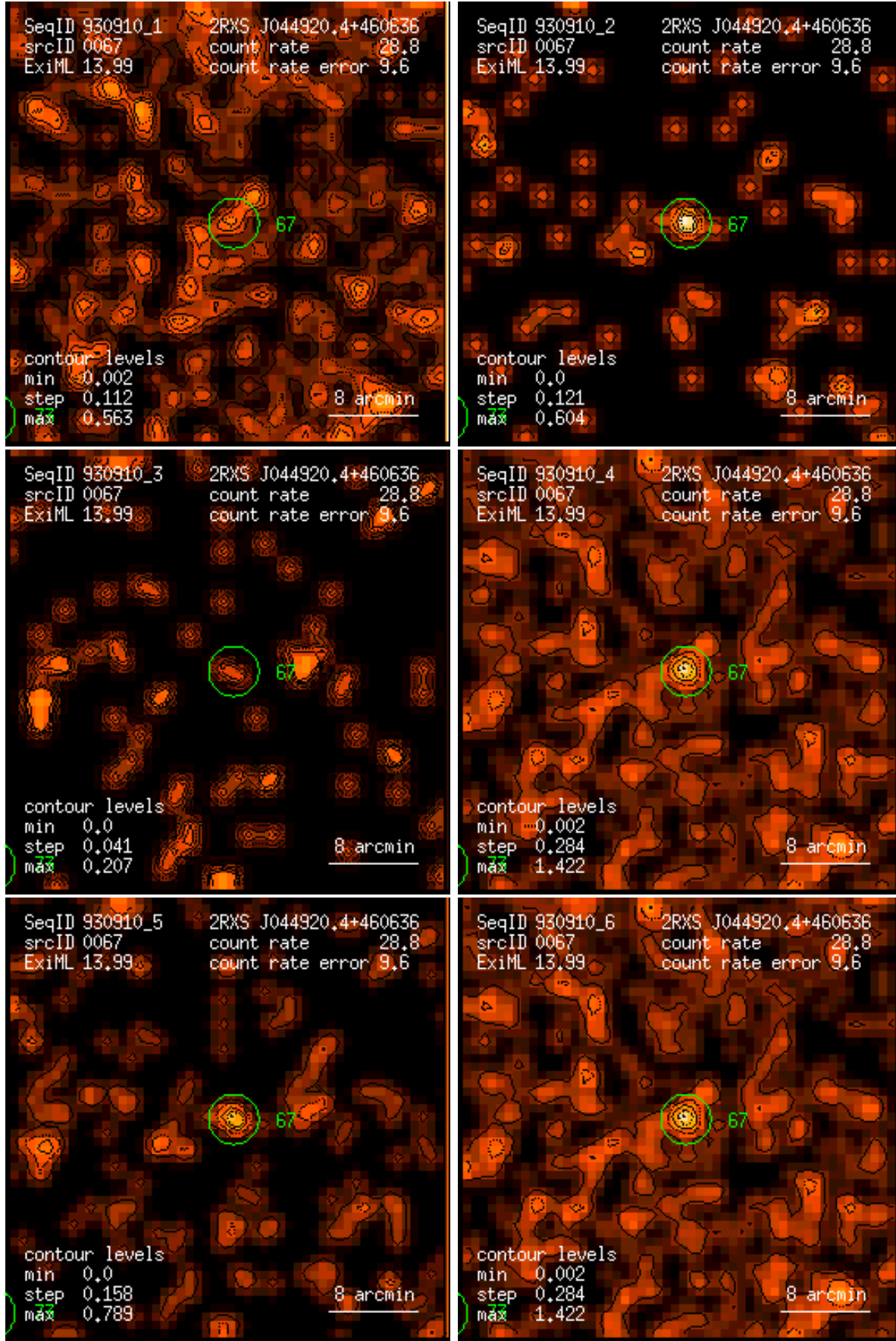
Figure 67: RASS 930910: detection 0067: band rate images, Gaussian filter: (1) PSPC channels 11 – 41, (2) 52 – 90, (3) 91 – 201, (4) 11 – 235, (5) 52 – 201, (6) 11 – 201. Broad band rates in counts/ks. Band rate contour levels in counts/ks/arcmin 2 .
