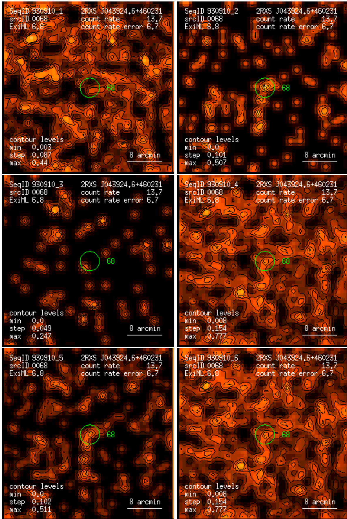
Figure 68: RASS 930910: detection 0068: band rate images, Gaussian filter: (1) PSPC channels 11 – 41, (2) 52 – 90, (3) 91 – 201, (4) 11 – 235, (5) 52 – 201, (6) 11 – 201. Broad band rates in counts/ks. Band rate contour levels in counts/ks/arcmin 2 .
