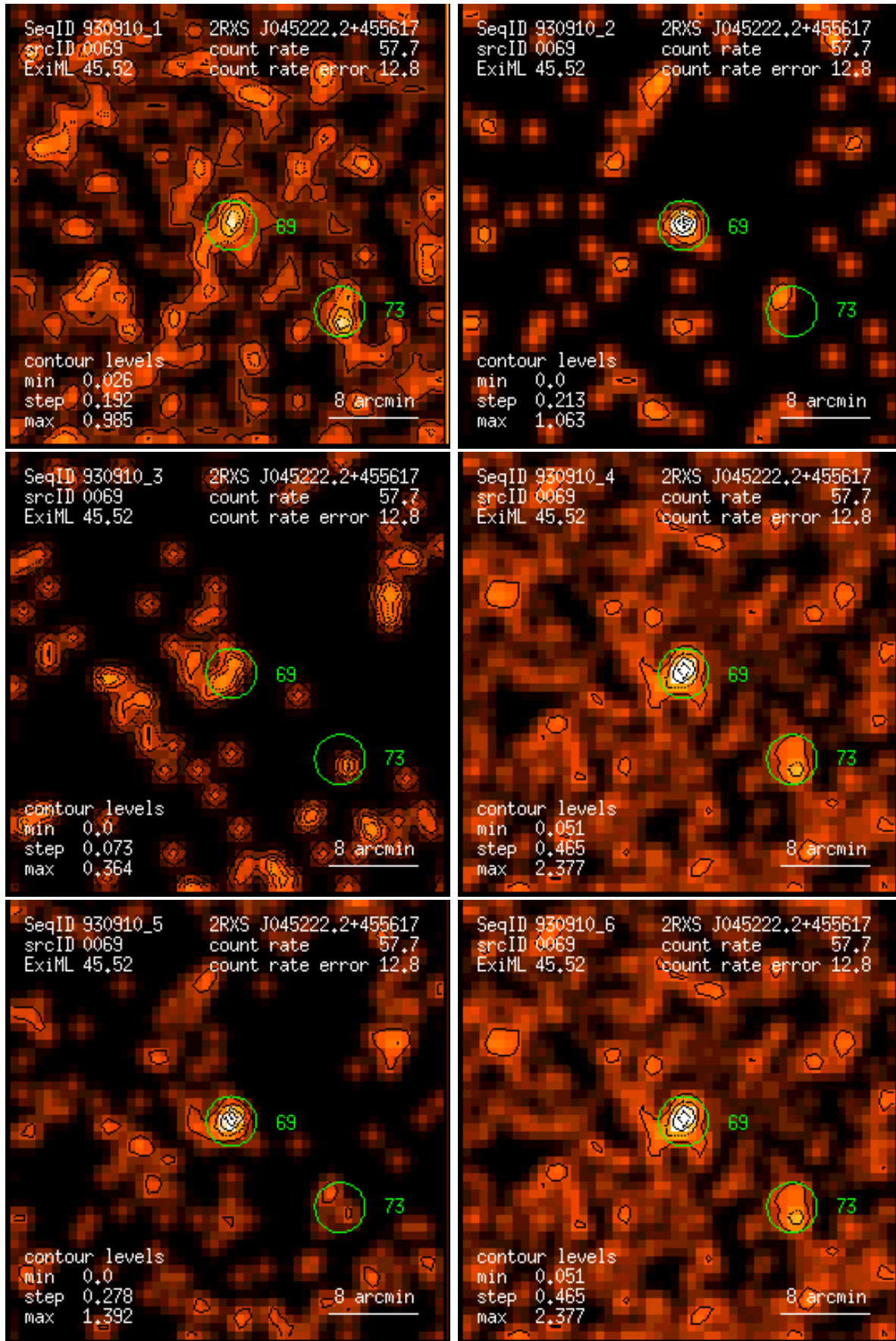
Figure 69: RASS 930910: detection 0069: band rate images, Gaussian filter: (1) PSPC channels 11 – 41, (2) 52 – 90, (3) 91 – 201, (4) 11 – 235, (5) 52 – 201, (6) 11 – 201. Broad band rates in counts/ks. Band rate contour levels in counts/ks/arcmin 2 .
