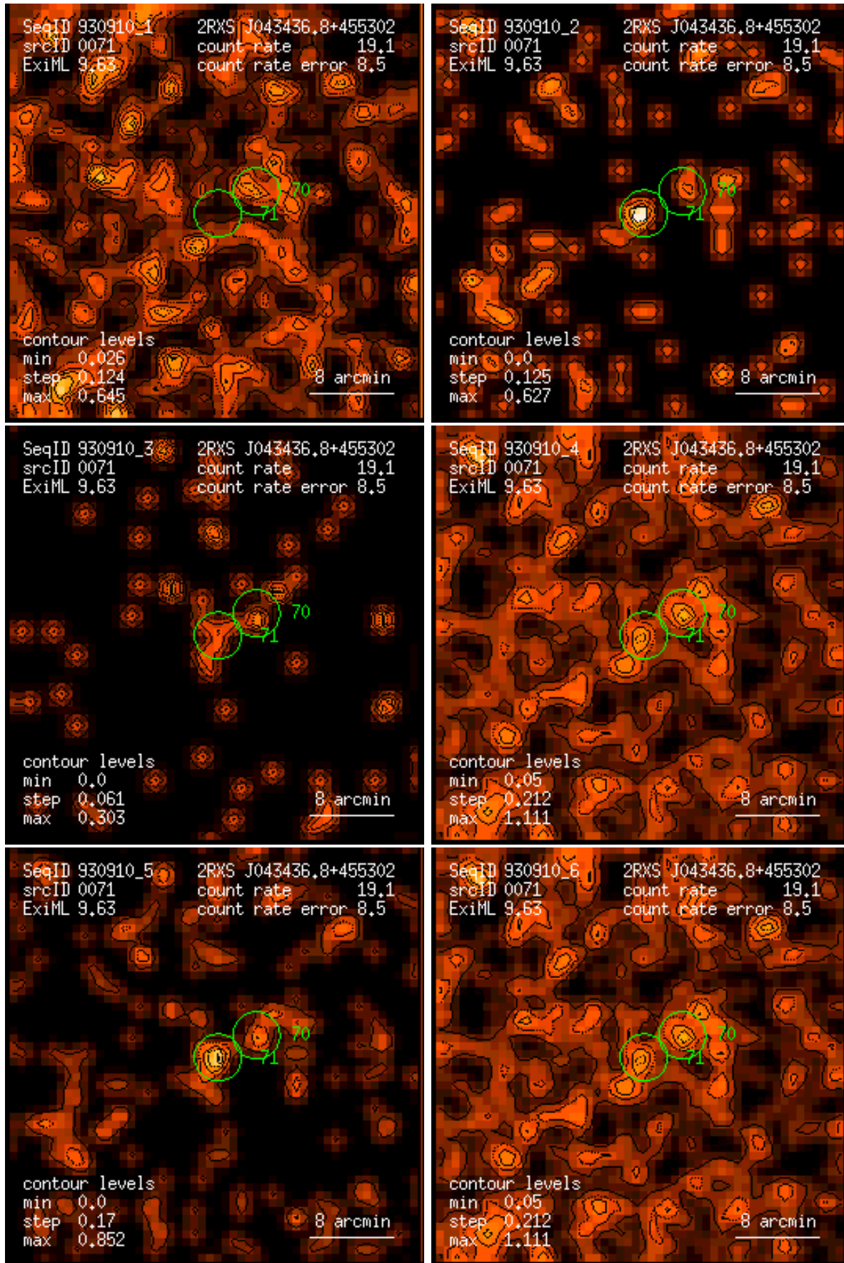
Figure 71: RASS 930910: detection 0071: band rate images, Gaussian filter: (1) PSPC channels 11 – 41, (2) 52 – 90, (3) 91 – 201, (4) 11 – 235, (5) 52 – 201, (6) 11 – 201. Broad band rates in counts/ks. Band rate contour levels in counts/ks/arcmin 2 .
