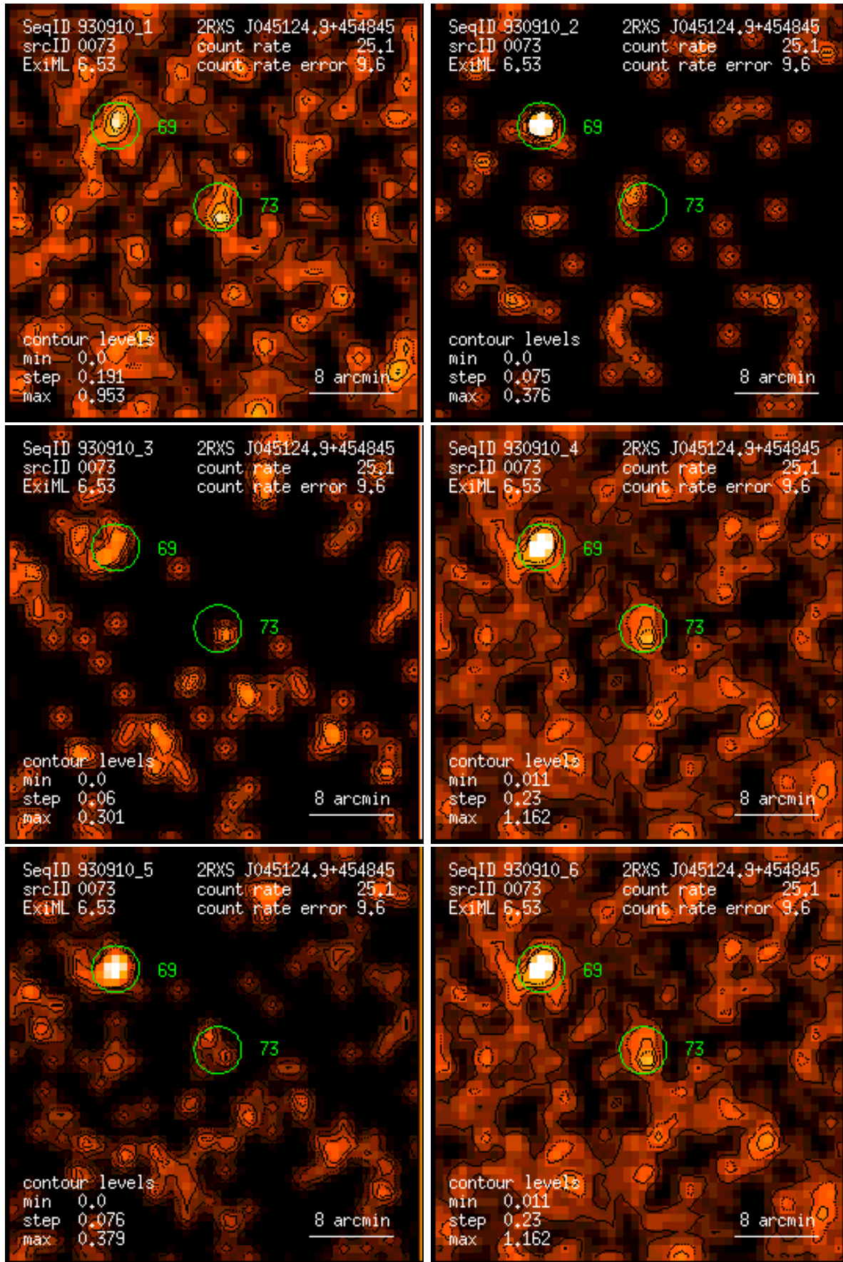
Figure 73: RASS 930910: detection 0073: band rate images, Gaussian filter: (1) PSPC channels 11 – 41, (2) 52 – 90, (3) 91 – 201, (4) 11 – 235, (5) 52 – 201, (6) 11 – 201. Broad band rates in counts/ks. Band rate contour levels in counts/ks/arcmin 2 .
