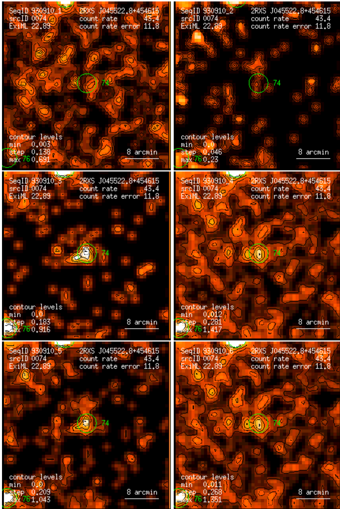
Figure 74: RASS 930910: detection 0074: band rate images, Gaussian filter: (1) PSPC channels 11 – 41, (2) 52 – 90, (3) 91 – 201, (4) 11 – 235, (5) 52 – 201, (6) 11 – 201. Broad band rates in counts/ks. Band rate contour levels in counts/ks/arcmin 2 .
