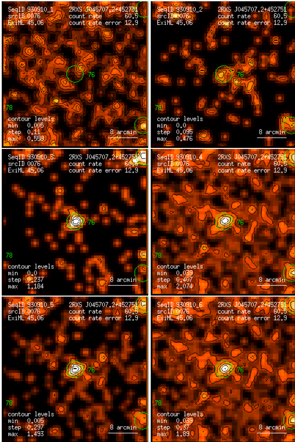
Figure 76: RASS 930910: detection 0076: band rate images, Gaussian filter: (1) PSPC channels 11 – 41, (2) 52 – 90, (3) 91 – 201, (4) 11 – 235, (5) 52 – 201, (6) 11 – 201. Broad band rates in counts/ks. Band rate contour levels in counts/ks/arcmin 2 .
