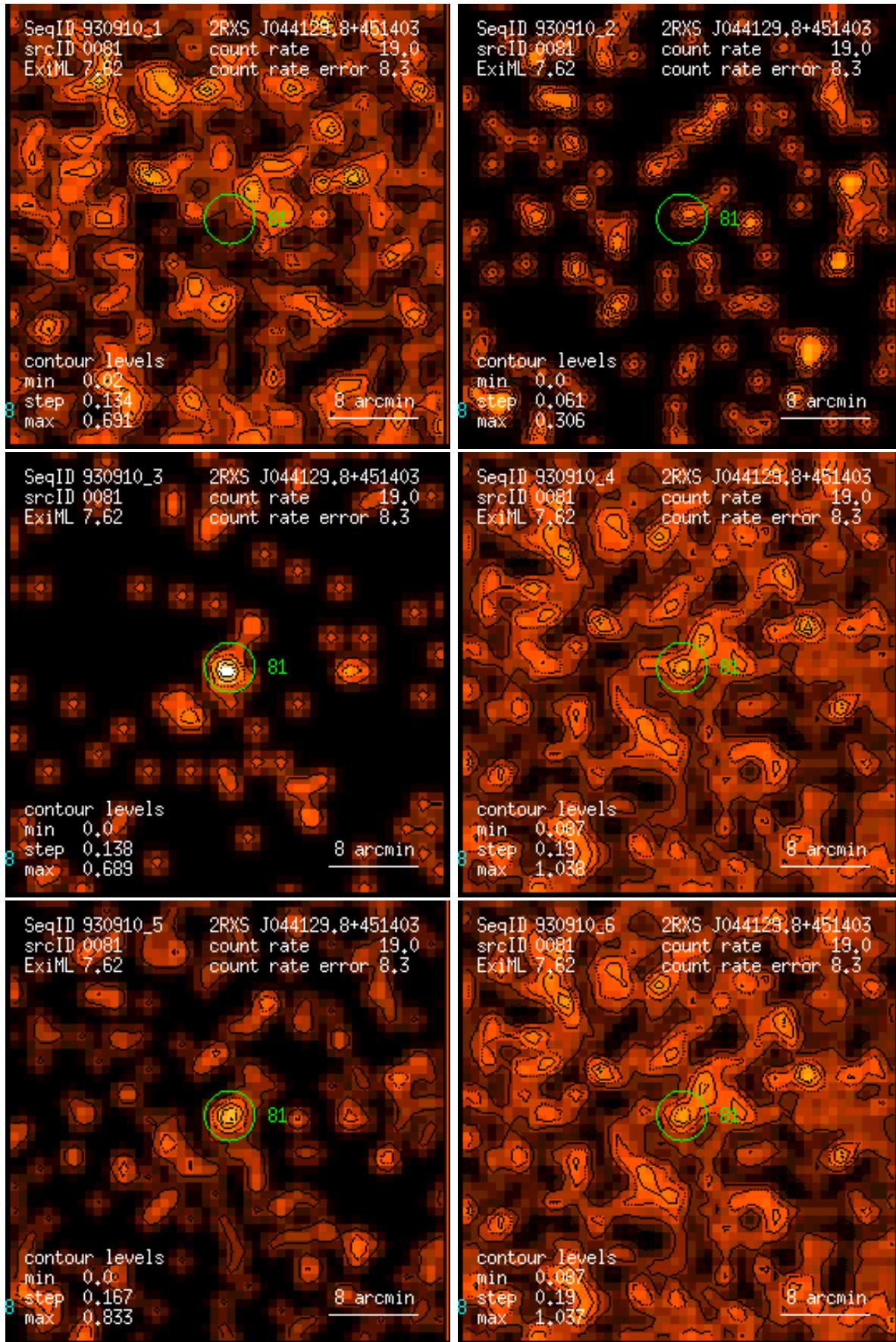
Figure 81: RASS 930910: detection 0081: band rate images, Gaussian filter: (1) PSPC channels 11 – 41, (2) 52 – 90, (3) 91 – 201, (4) 11 – 235, (5) 52 – 201, (6) 11 – 201. Broad band rates in counts/ks. Band rate contour levels in counts/ks/arcmin 2 .
