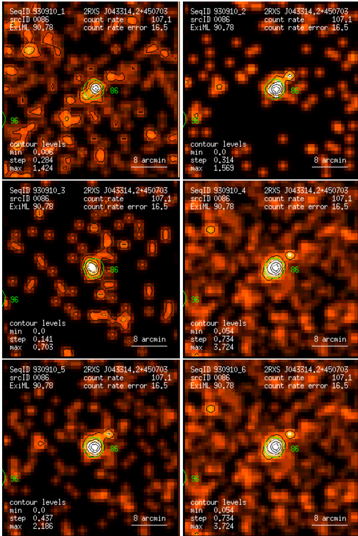
Figure 86: RASS 930910: detection 0086: band rate images, Gaussian filter: (1) PSPC channels 11 – 41, (2) 52 – 90, (3) 91 – 201, (4) 11 – 235, (5) 52 – 201, (6) 11 – 201. Broad band rates in counts/ks. Band rate contour levels in counts/ks/arcmin 2 .
