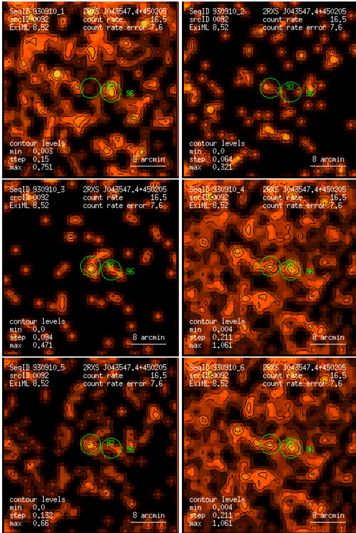
Figure 92: RASS 930910: detection 0092: band rate images, Gaussian filter: (1) PSPC channels 11 – 41, (2) 52 – 90, (3) 91 – 201, (4) 11 – 235, (5) 52 – 201, (6) 11 – 201. Broad band rates in counts/ks. Band rate contour levels in counts/ks/arcmin 2 .
