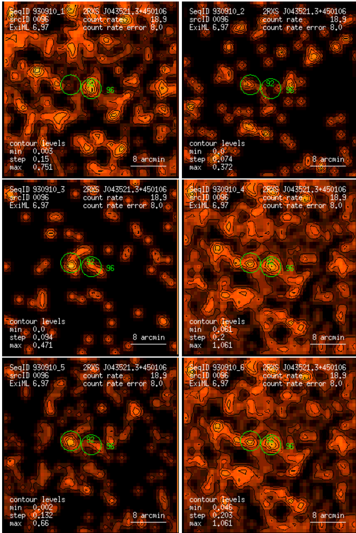
Figure 96: RASS 930910: detection 0096: band rate images, Gaussian filter: (1) PSPC channels 11 – 41, (2) 52 – 90, (3) 91 – 201, (4) 11 – 235, (5) 52 – 201, (6) 11 – 201. Broad band rates in counts/ks. Band rate contour levels in counts/ks/arcmin 2 .
