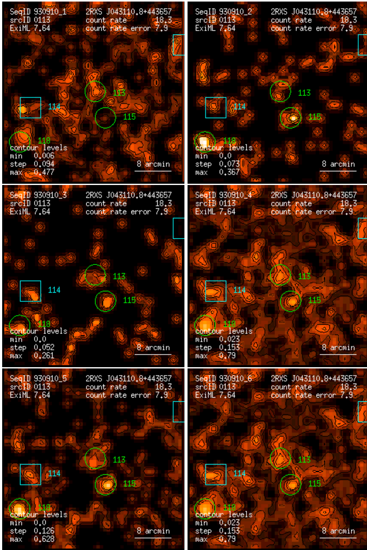
Figure 113: RASS 930910: detection 0113: band rate images, Gaussian filter: (1) PSPC channels 11 – 41, (2) 52 – 90, (3) 91 – 201, (4) 11 – 235, (5) 52 – 201, (6) 11 – 201. Broad band rates in counts/ks. Band rate contour levels in counts/ks/arcmin 2 .
