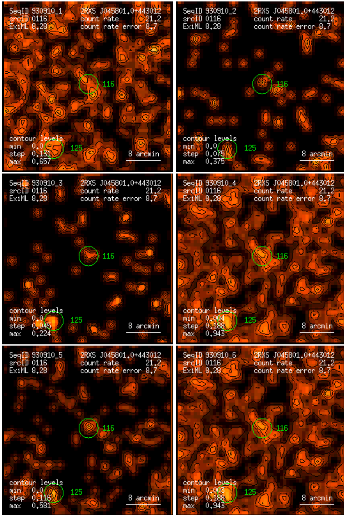
Figure 116: RASS 930910: detection 0116: band rate images, Gaussian filter: (1) PSPC channels 11 – 41, (2) 52 – 90, (3) 91 – 201, (4) 11 – 235, (5) 52 – 201, (6) 11 – 201. Broad band rates in counts/ks. Band rate contour levels in counts/ks/arcmin 2 .
