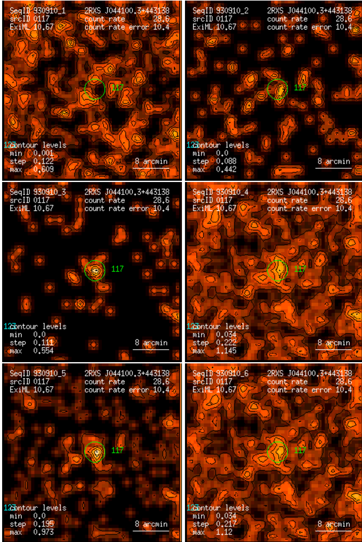
Figure 117: RASS 930910: detection 0117: band rate images, Gaussian filter: (1) PSPC channels 11 – 41, (2) 52 – 90, (3) 91 – 201, (4) 11 – 235, (5) 52 – 201, (6) 11 – 201. Broad band rates in counts/ks. Band rate contour levels in counts/ks/arcmin 2 .
