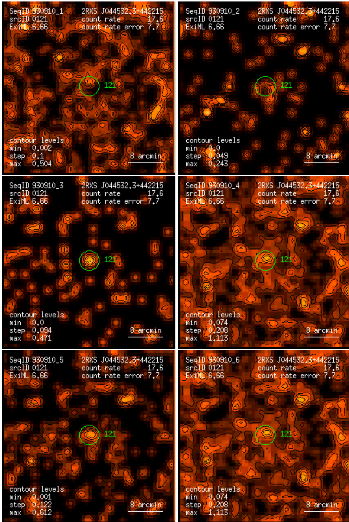
Figure 121: RASS 930910: detection 0121: band rate images, Gaussian filter: (1) PSPC channels 11 – 41, (2) 52 – 90, (3) 91 – 201, (4) 11 – 235, (5) 52 – 201, (6) 11 – 201. Broad band rates in counts/ks. Band rate contour levels in counts/ks/arcmin 2 .
