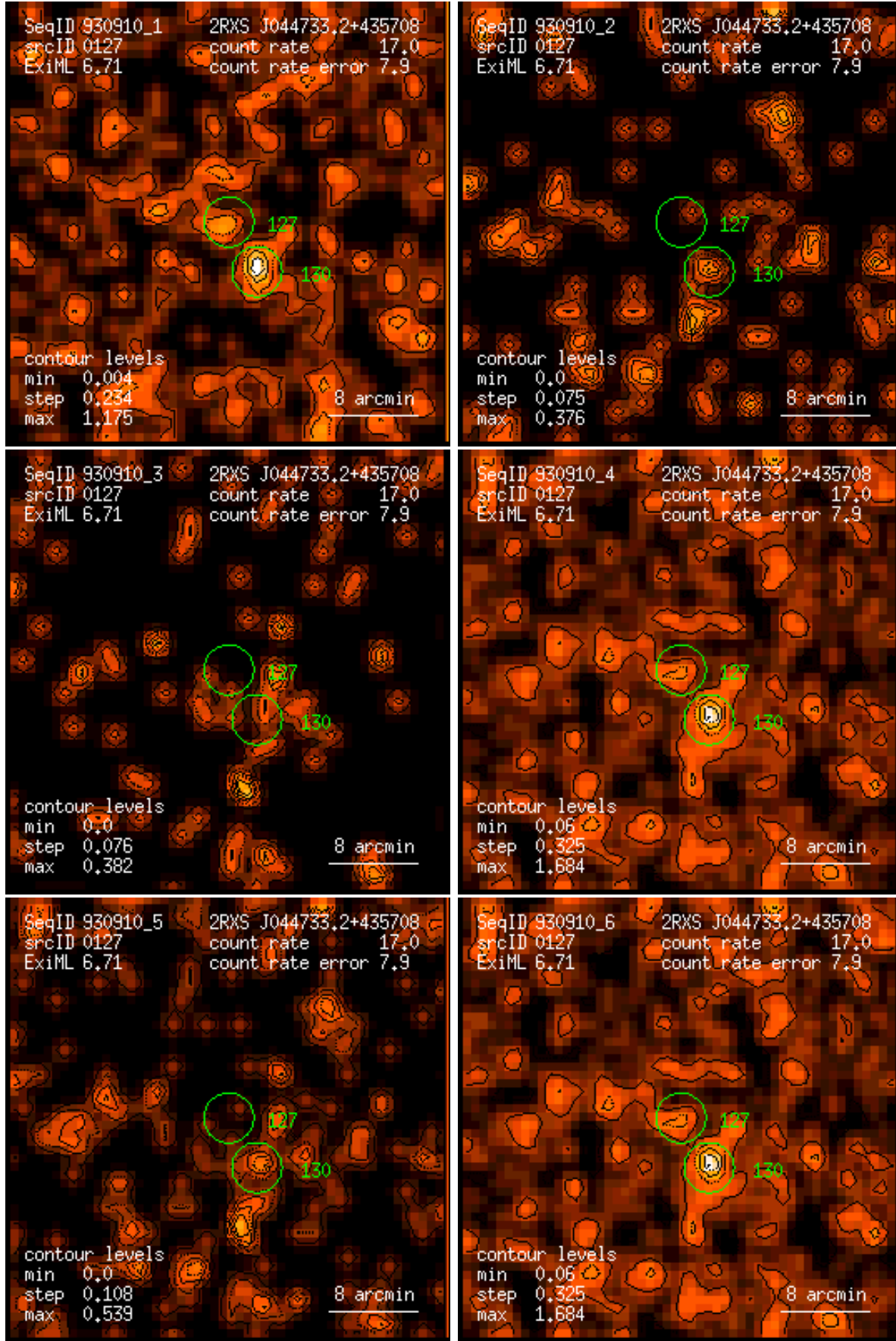
Figure 127: RASS 930910: detection 0127: band rate images, Gaussian filter: (1) PSPC channels 11 – 41, (2) 52 – 90, (3) 91 – 201, (4) 11 – 235, (5) 52 – 201, (6) 11 – 201. Broad band rates in counts/ks. Band rate contour levels in counts/ks/arcmin 2 .
