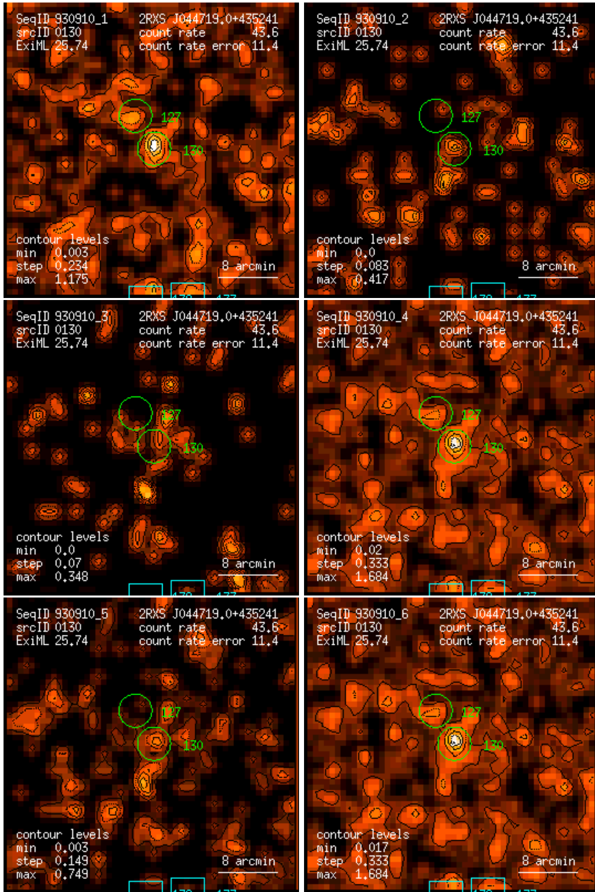
Figure 130: RASS 930910: detection 0130: band rate images, Gaussian filter: (1) PSPC channels 11 – 41, (2) 52 – 90, (3) 91 – 201, (4) 11 – 235, (5) 52 – 201, (6) 11 – 201. Broad band rates in counts/ks. Band rate contour levels in counts/ks/arcmin 2 .
