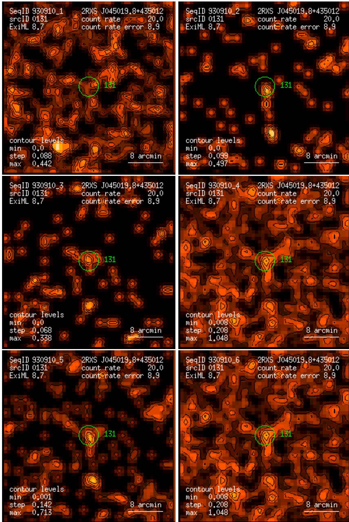
Figure 131: RASS 930910: detection 0131: band rate images, Gaussian filter: (1) PSPC channels 11 – 41, (2) 52 – 90, (3) 91 – 201, (4) 11 – 235, (5) 52 – 201, (6) 11 – 201. Broad band rates in counts/ks. Band rate contour levels in counts/ks/arcmin 2 .
