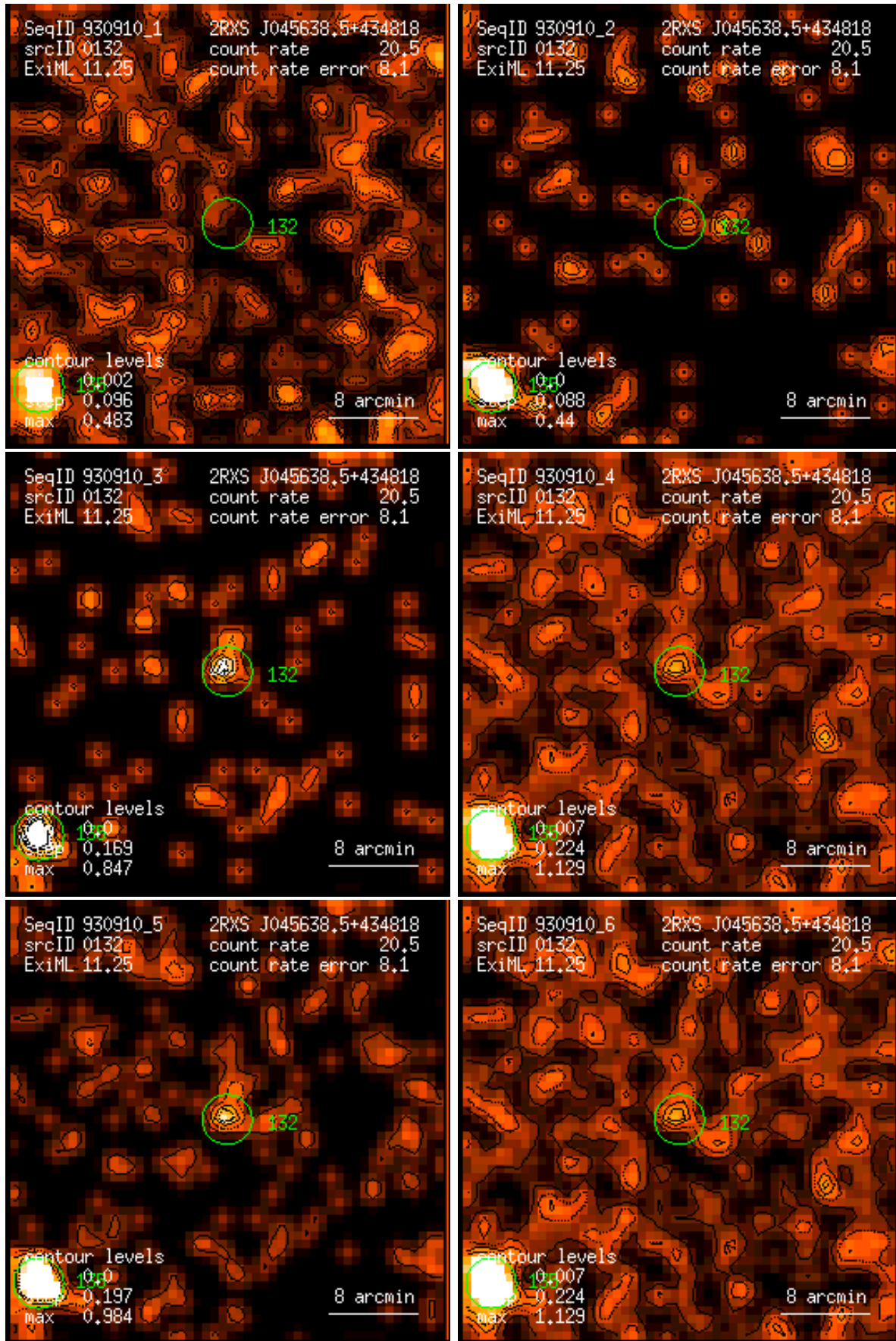
Figure 132: RASS 930910: detection 0132: band rate images, Gaussian filter: (1) PSPC channels 11 – 41, (2) 52 – 90, (3) 91 – 201, (4) 11 – 235, (5) 52 – 201, (6) 11 – 201. Broad band rates in counts/ks. Band rate contour levels in counts/ks/arcmin 2 .
