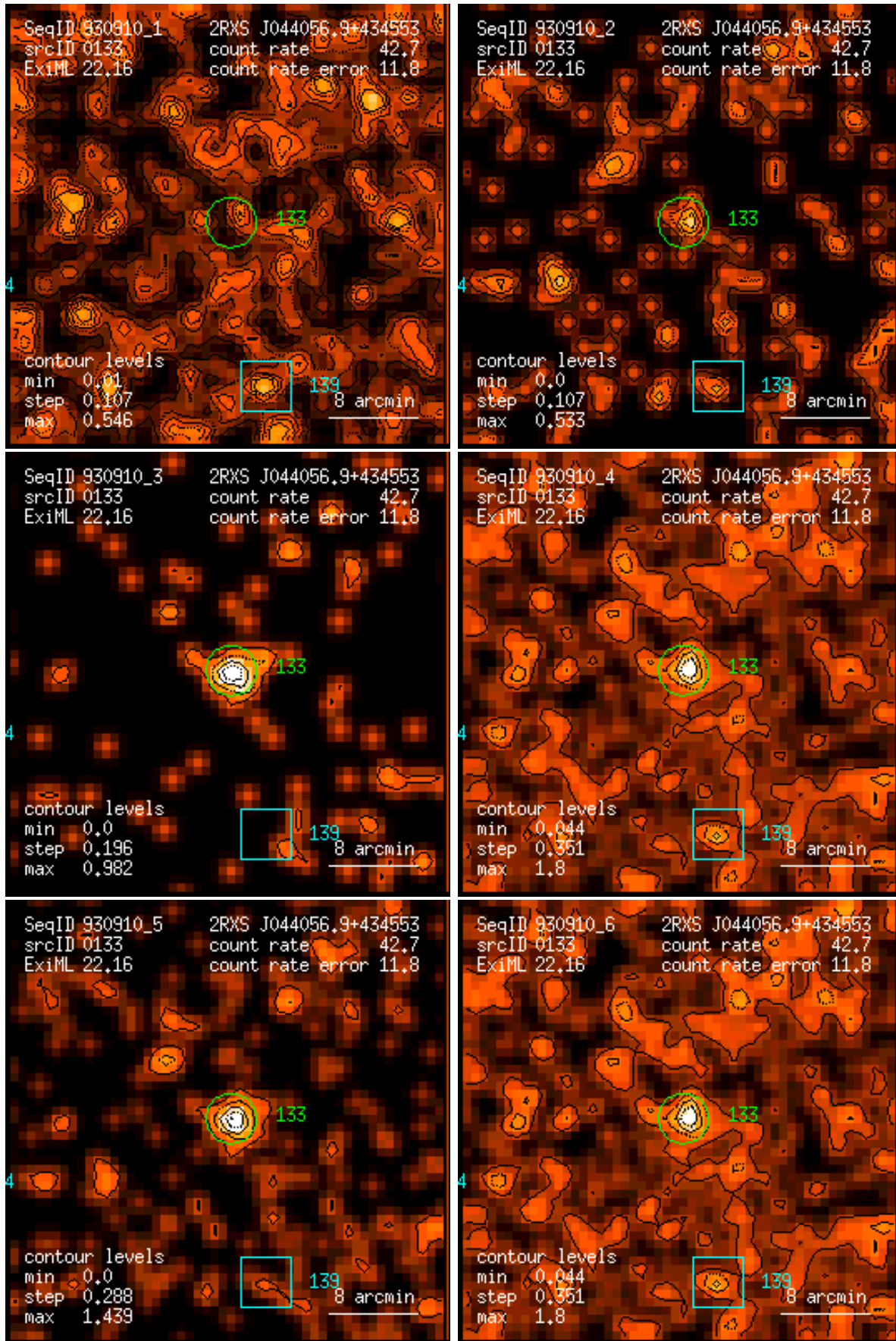
Figure 133: RASS 930910: detection 0133: band rate images, Gaussian filter: (1) PSPC channels 11 – 41, (2) 52 – 90, (3) 91 – 201, (4) 11 – 235, (5) 52 – 201, (6) 11 – 201. Broad band rates in counts/ks. Band rate contour levels in counts/ks/arcmin 2 .
