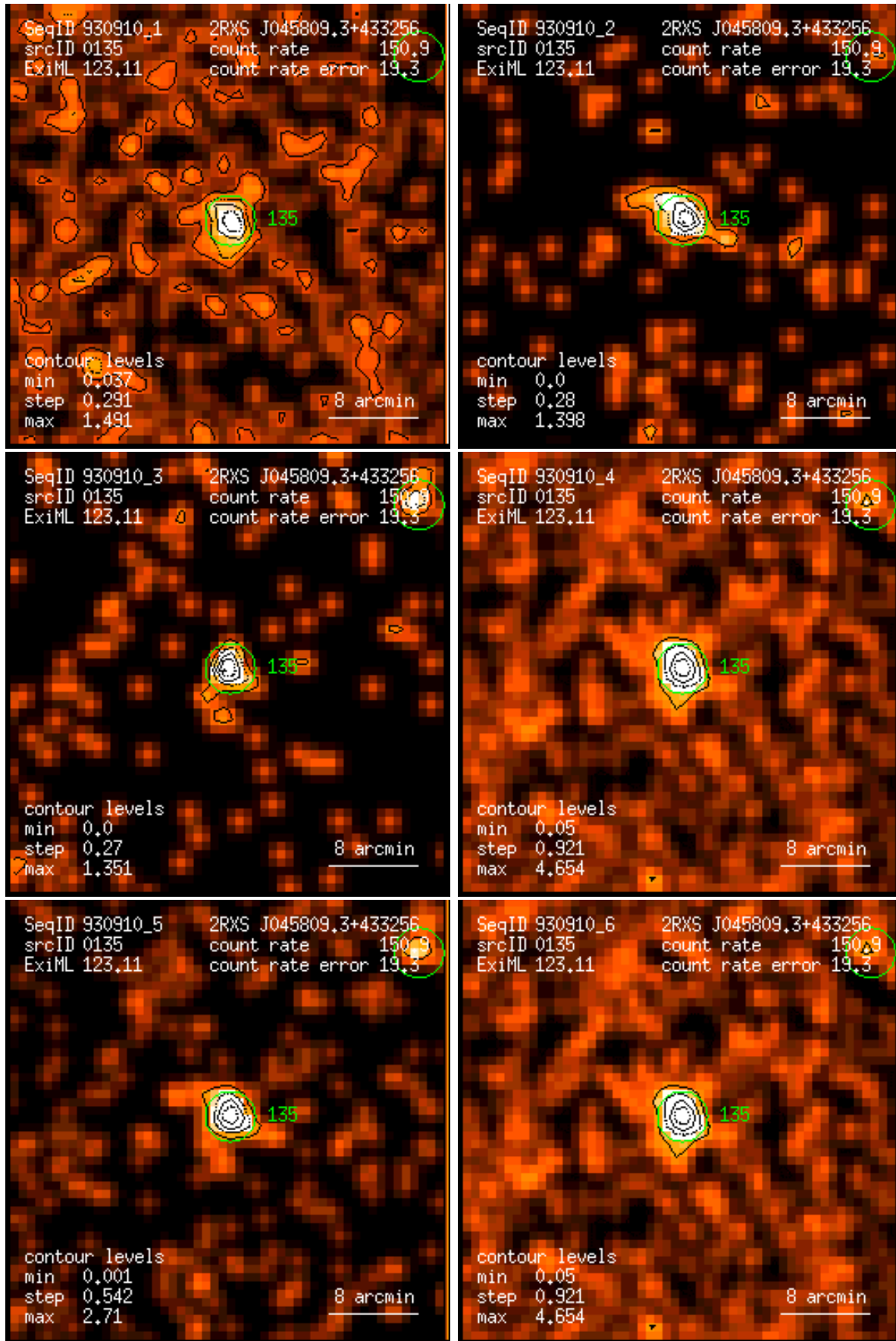
Figure 135: RASS 930910: detection 0135: band rate images, Gaussian filter: (1) PSPC channels 11 – 41, (2) 52 – 90, (3) 91 – 201, (4) 11 – 235, (5) 52 – 201, (6) 11 – 201. Broad band rates in counts/ks. Band rate contour levels in counts/ks/arcmin 2 .
