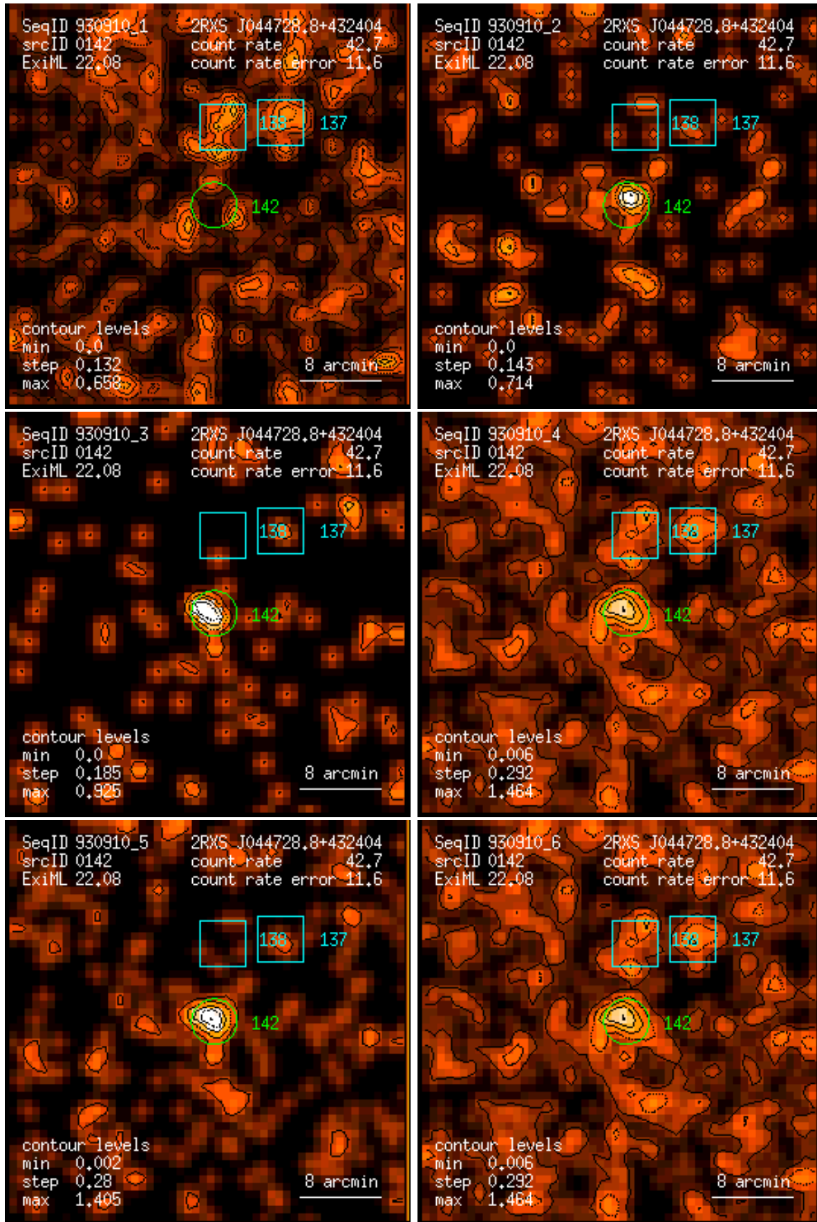
Figure 142: RASS 930910: detection 0142: band rate images, Gaussian filter: (1) PSPC channels 11 – 41, (2) 52 – 90, (3) 91 – 201, (4) 11 – 235, (5) 52 – 201, (6) 11 – 201. Broad band rates in counts/ks. Band rate contour levels in counts/ks/arcmin 2 .
