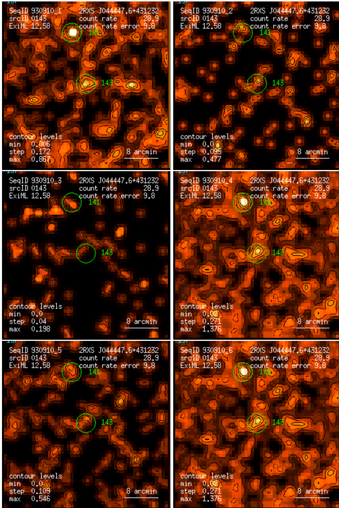
Figure 143: RASS 930910: detection 0143: band rate images, Gaussian filter: (1) PSPC channels 11 – 41, (2) 52 – 90, (3) 91 – 201, (4) 11 – 235, (5) 52 – 201, (6) 11 – 201. Broad band rates in counts/ks. Band rate contour levels in counts/ks/arcmin 2 .
