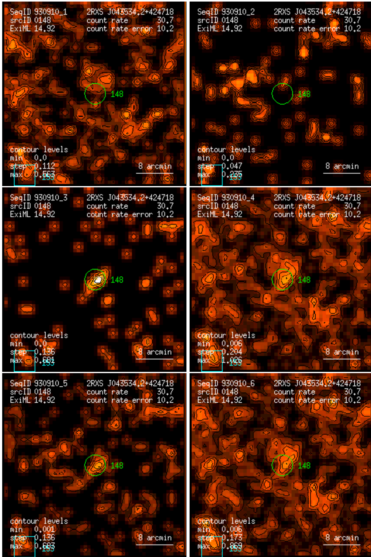
Figure 148: RASS 930910: detection 0148: band rate images, Gaussian filter: (1) PSPC channels 11 – 41, (2) 52 – 90, (3) 91 – 201, (4) 11 – 235, (5) 52 – 201, (6) 11 – 201. Broad band rates in counts/ks. Band rate contour levels in counts/ks/arcmin 2 .
