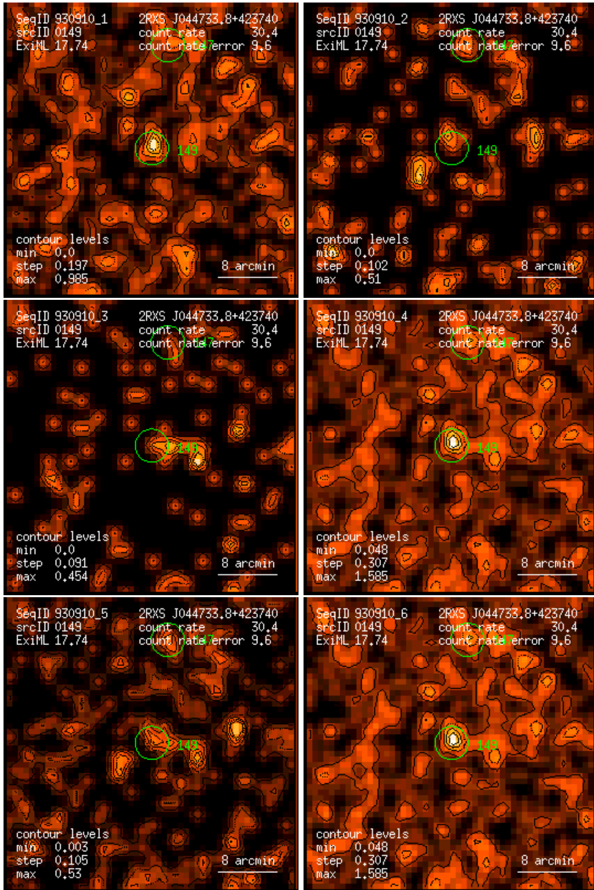
Figure 149: RASS 930910: detection 0149: band rate images, Gaussian filter: (1) PSPC channels 11 – 41, (2) 52 – 90, (3) 91 – 201, (4) 11 – 235, (5) 52 – 201, (6) 11 – 201. Broad band rates in counts/ks. Band rate contour levels in counts/ks/arcmin 2 .
