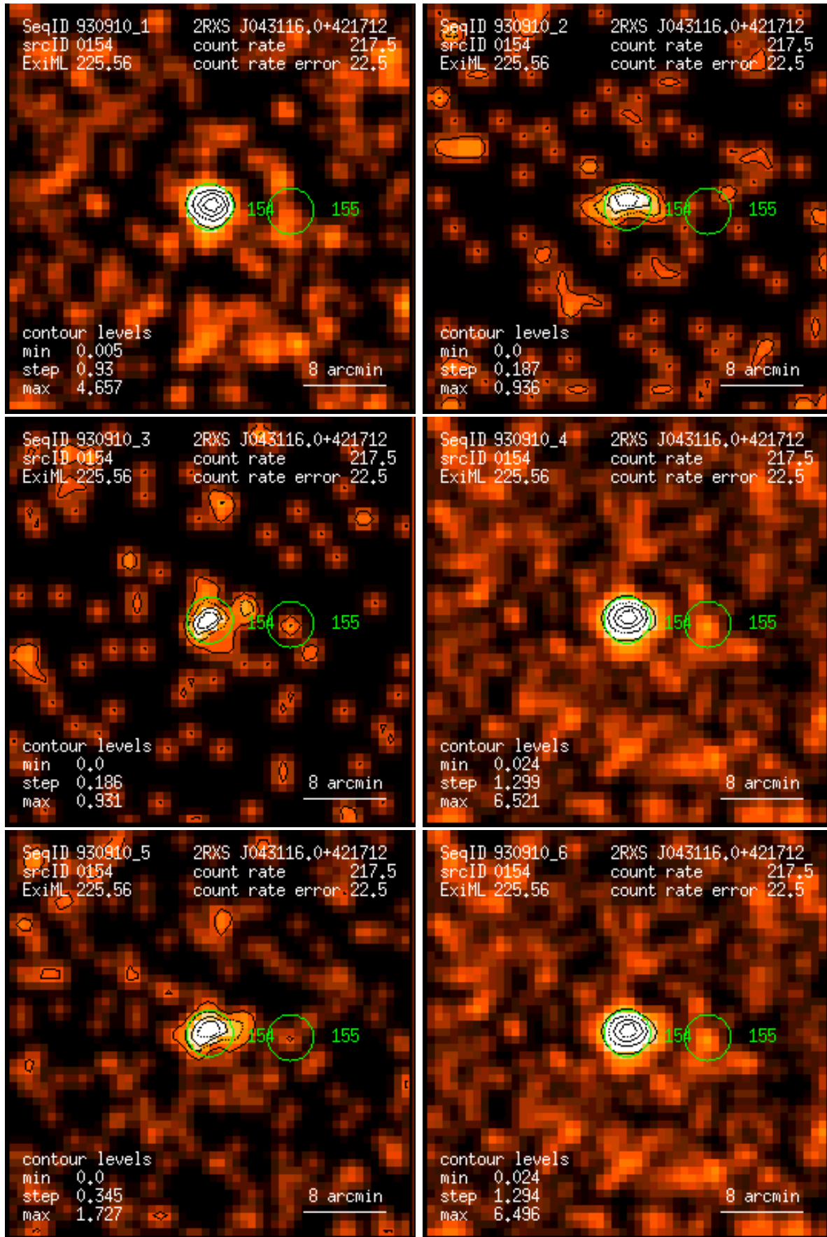
Figure 154: RASS 930910: detection 0154: band rate images, Gaussian filter: (1) PSPC channels 11 – 41, (2) 52 – 90, (3) 91 – 201, (4) 11 – 235, (5) 52 – 201, (6) 11 – 201. Broad band rates in counts/ks. Band rate contour levels in counts/ks/arcmin 2 .
