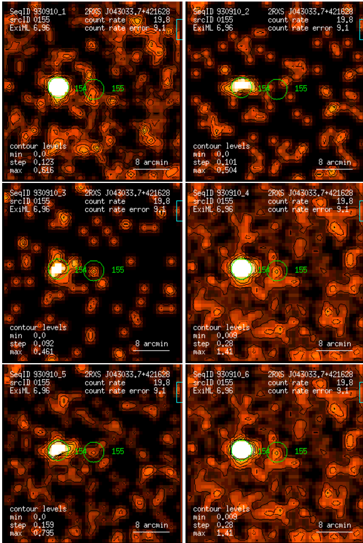
Figure 155: RASS 930910: detection 0155: band rate images, Gaussian filter: (1) PSPC channels 11 – 41, (2) 52 – 90, (3) 91 – 201, (4) 11 – 235, (5) 52 – 201, (6) 11 – 201. Broad band rates in counts/ks. Band rate contour levels in counts/ks/arcmin 2 .
