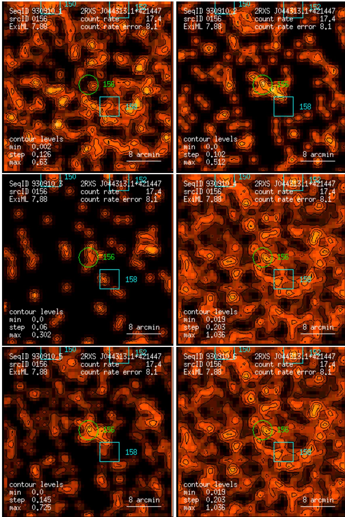
Figure 156: RASS 930910: detection 0156: band rate images, Gaussian filter: (1) PSPC channels 11 – 41, (2) 52 – 90, (3) 91 – 201, (4) 11 – 235, (5) 52 – 201, (6) 11 – 201. Broad band rates in counts/ks. Band rate contour levels in counts/ks/arcmin 2 .
