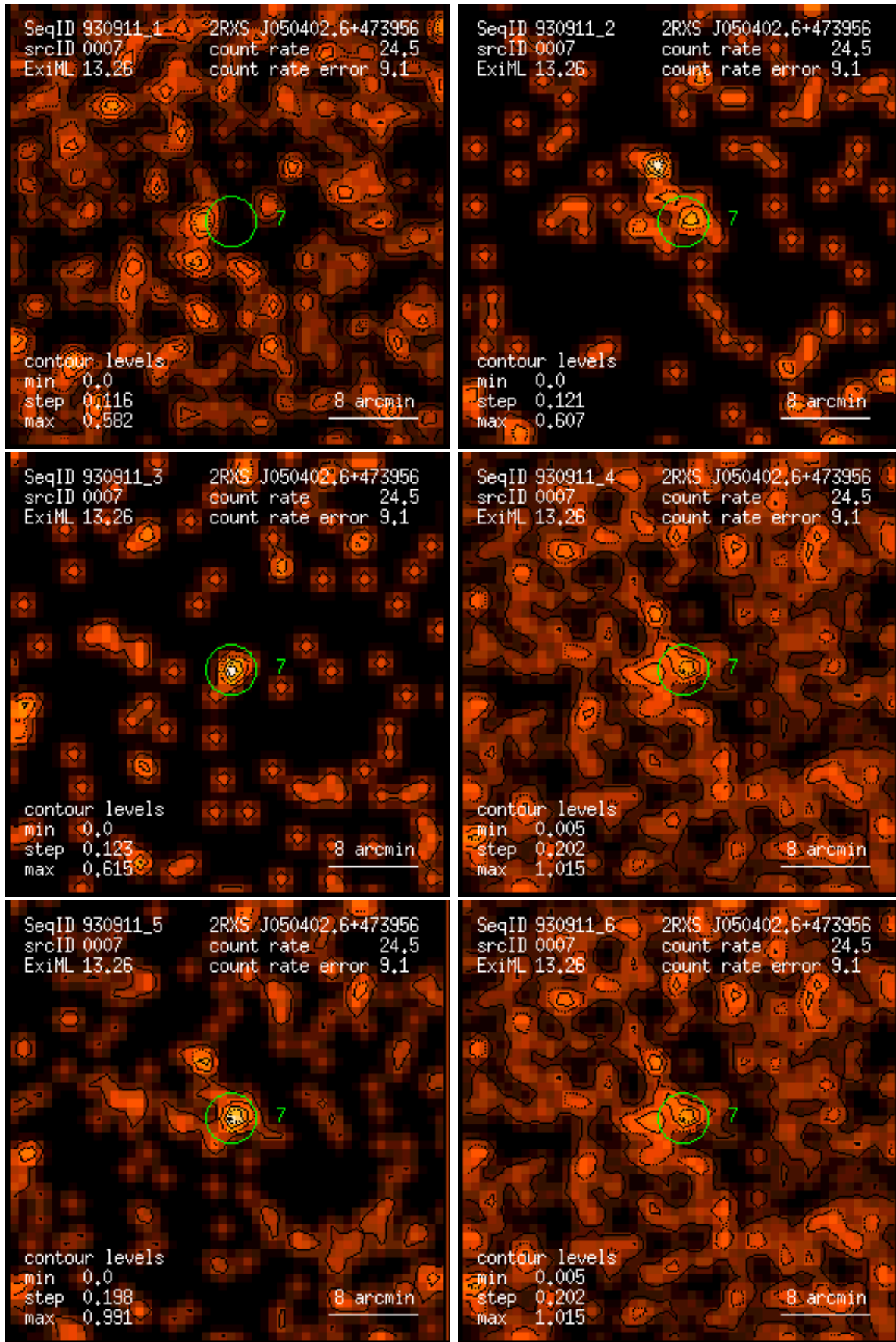
Figure 7: RASS 930911: detection 0007: band rate images, Gaussian filter: (1) PSPC channels 11 – 41, (2) 52 – 90, (3) 91 – 201, (4) 11 – 235, (5) 52 – 201, (6) 11 – 201. Broad band rates in counts/ks. Band rate contour levels in counts/ks/arcmin 2 .
