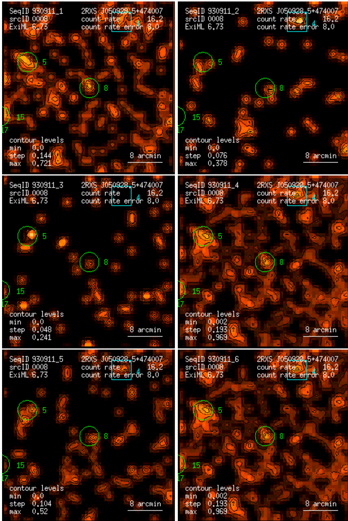
Figure 8: RASS 930911: detection 0008: band rate images, Gaussian filter: (1) PSPC channels 11 – 41, (2) 52 – 90, (3) 91 – 201, (4) 11 – 235, (5) 52 – 201, (6) 11 – 201. Broad band rates in counts/ks. Band rate contour levels in counts/ks/arcmin 2 .
