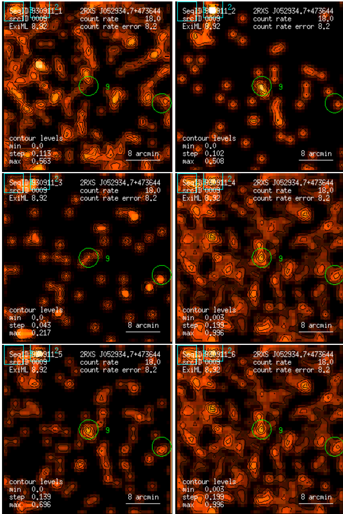
Figure 9: RASS 930911: detection 0009: band rate images, Gaussian filter: (1) PSPC channels 11 – 41, (2) 52 – 90, (3) 91 – 201, (4) 11 – 235, (5) 52 – 201, (6) 11 – 201. Broad band rates in counts/ks. Band rate contour levels in counts/ks/arcmin 2 .
