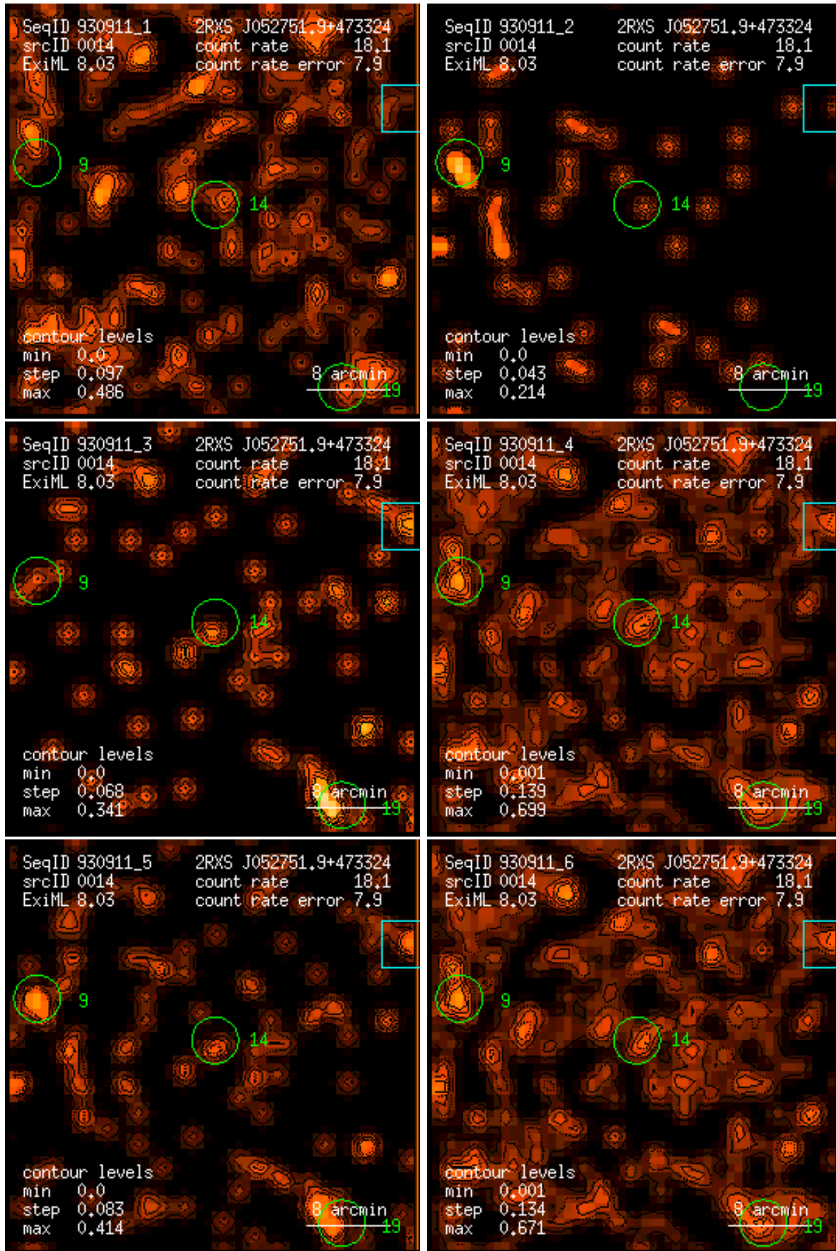
Figure 14: RASS 930911: detection 0014: band rate images, Gaussian filter: (1) PSPC channels 11 – 41, (2) 52 – 90, (3) 91 – 201, (4) 11 – 235, (5) 52 – 201, (6) 11 – 201. Broad band rates in counts/ks. Band rate contour levels in counts/ks/arcmin 2 .
